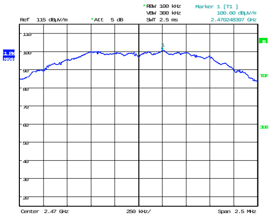
2470 MHz
