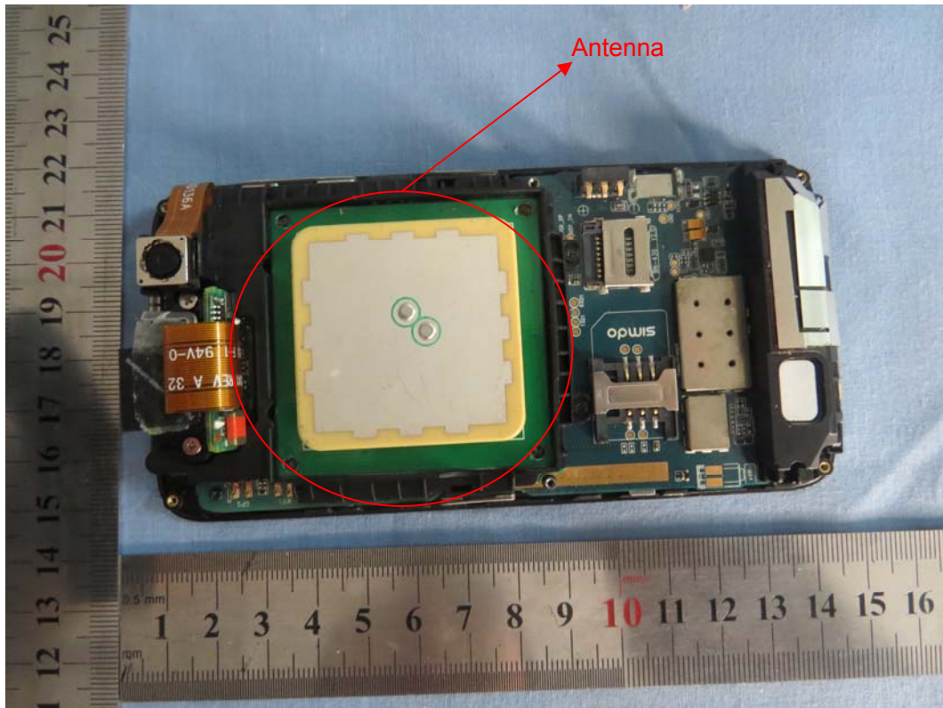
c. Antenna Schemes(Back Side of EUT)
