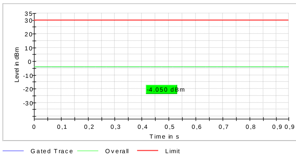
Screenshot: Output power. Middle channel. BLE.
