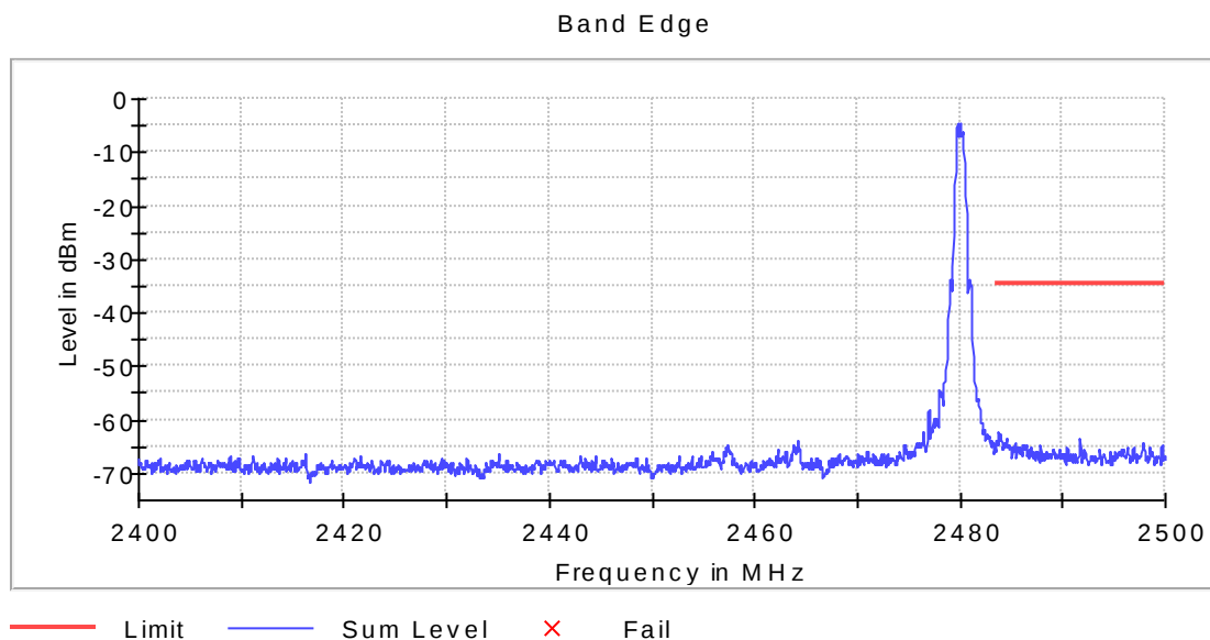
Screenshot: Upper band edge sweep. High channel. BLE.
