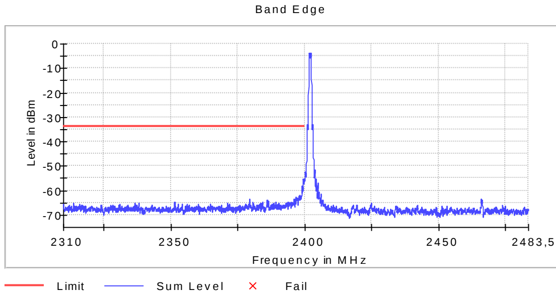
Screenshot: Lower band edge sweep. Low channel. BLE.
