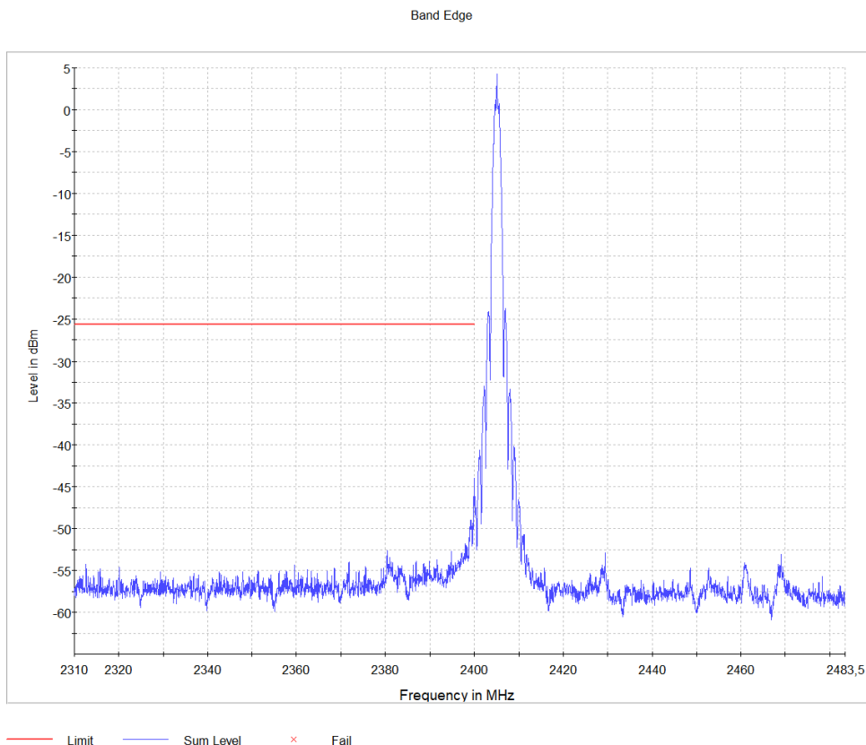
Screenshot: Lower band edge sweep. low channel
