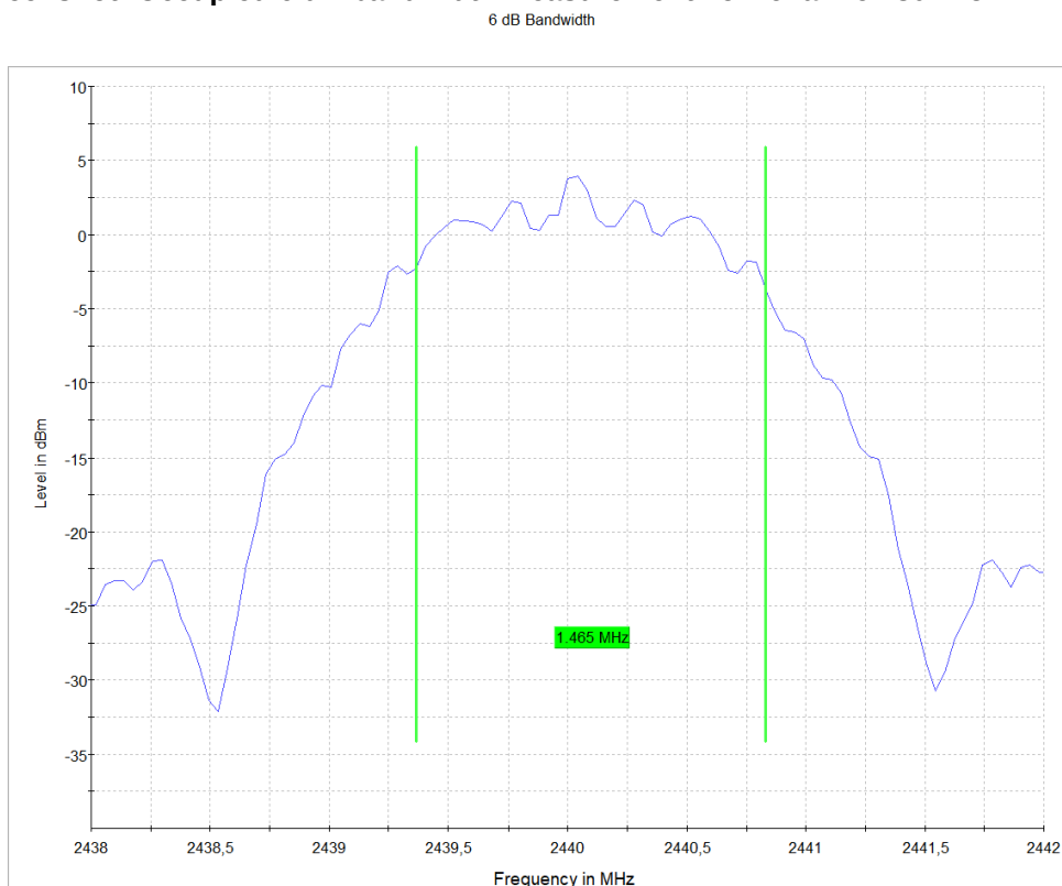
Screenshot: Occupied 6 dB bandwidth Measurement. middle channel. 802.15.4.
