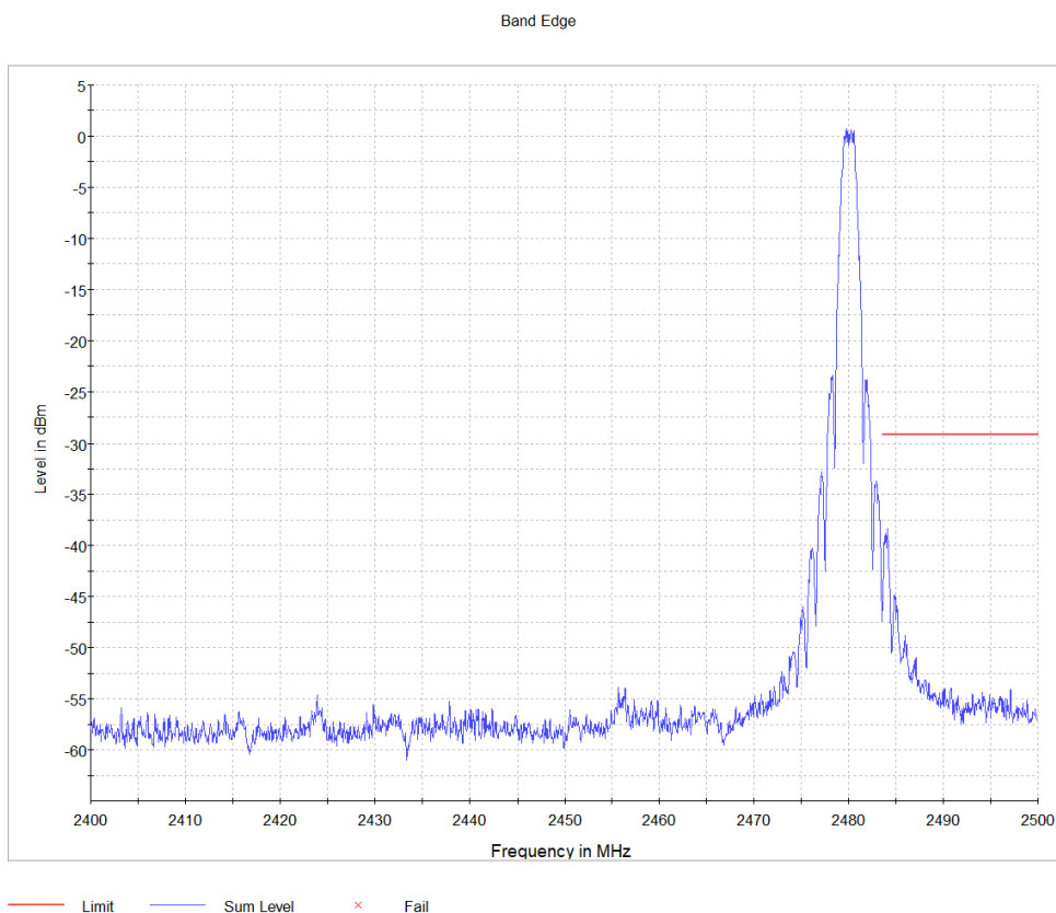
Screenshot: Upper band edge sweep. high channel
