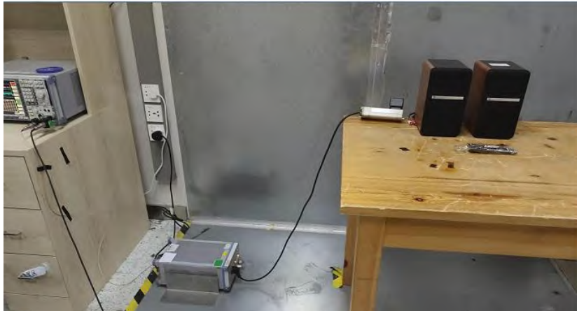
Radiated Emissions
