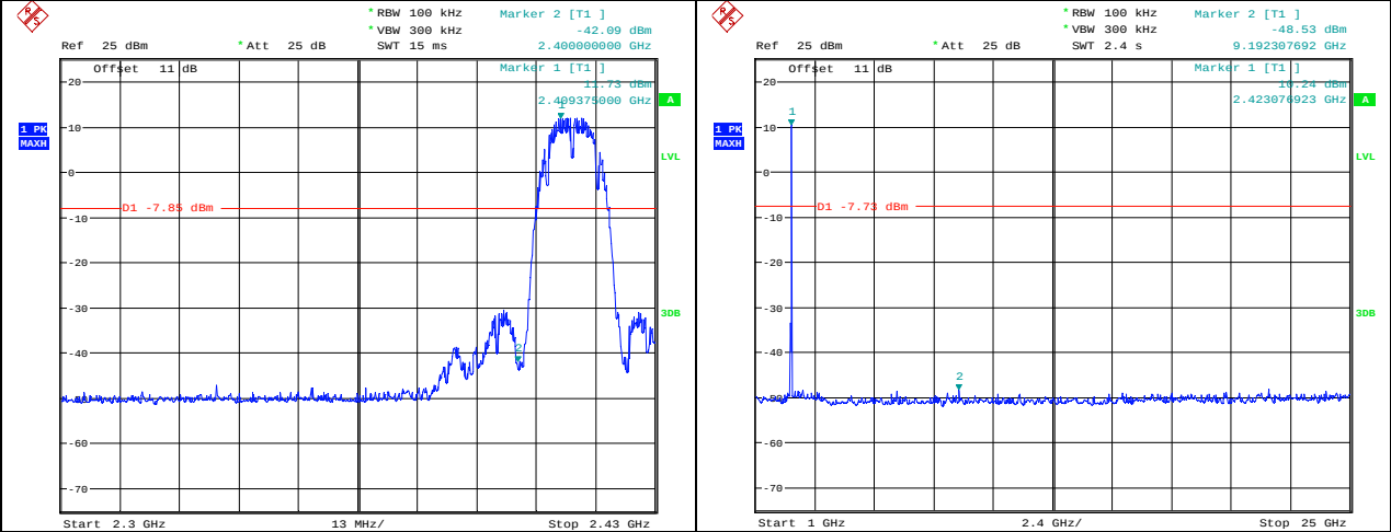
11g CH1
