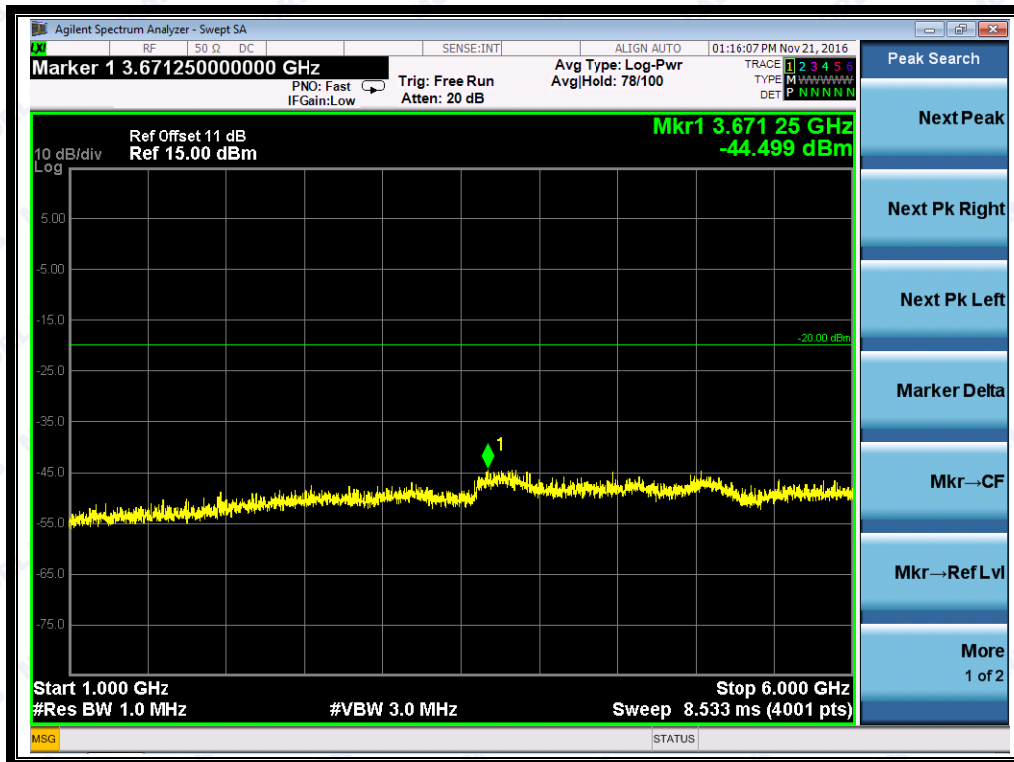
(Plot C7: FSK 434.5375MHz, 1GHz to 6GHz)
