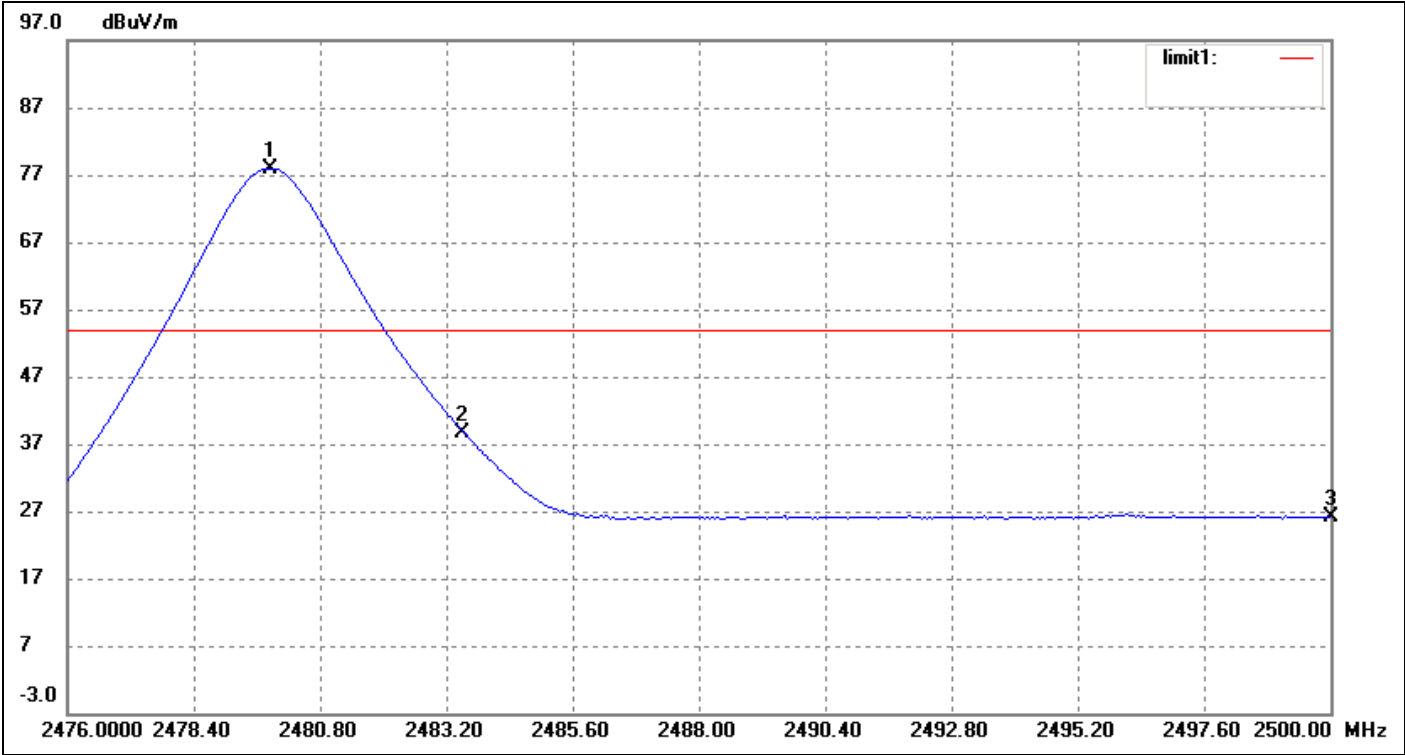
Highest Bandedge
