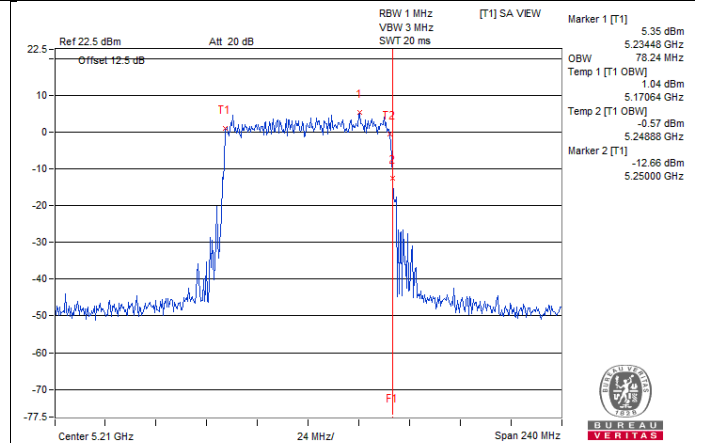
802.11ax (HE80+80) / Chain 7 : CH42
