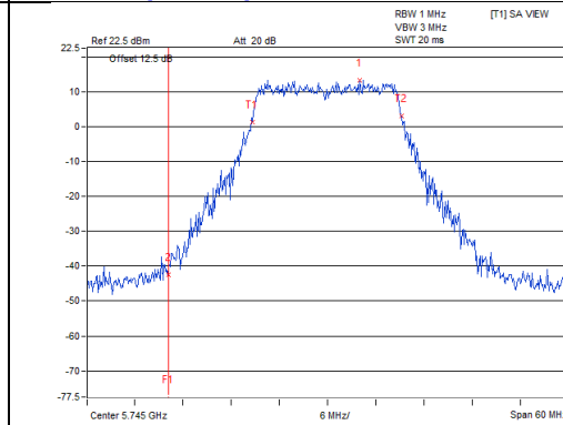
802.11ac (VHT20)_Chain 3 / CH149
