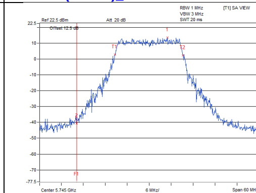
802.11ac (VHT20)_Chain 7 / CH149
