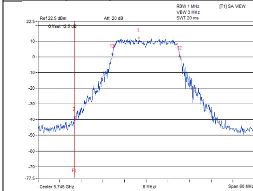
802.11ac (VHT20)_Chain 2 / CH149
