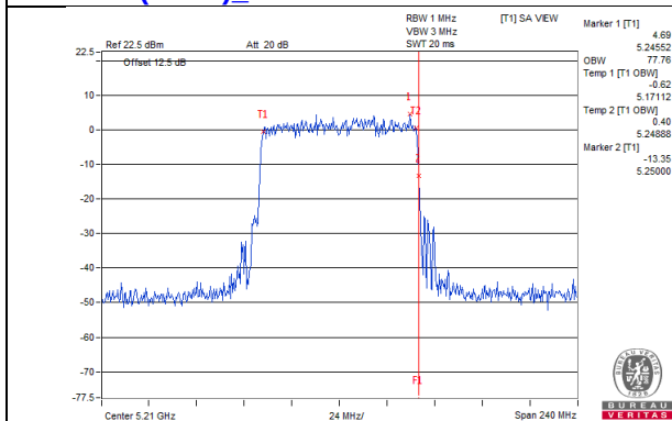
802.11ax (HE80)_Chain 6 / CH42
