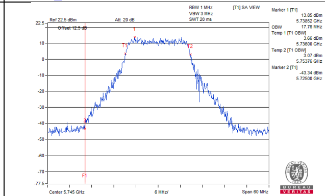
802.11a_Chain 3 / CH149
