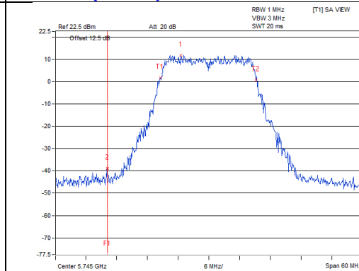
802.11ac (VHT20)_Chain 5 / CH149
