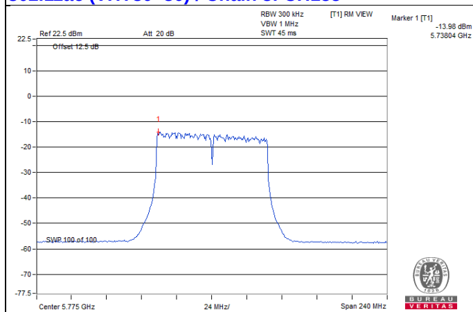
802.11ac (VHT80+80) / Chain 3: CH155
