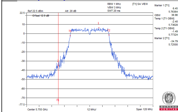
802.11ac (VHT40)_Chain 2 / CH151
