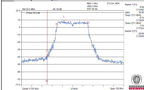
802.11ac (VHT40)_Chain 4 / CH151
