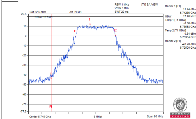
802.11a_Chain 2 / CH149
