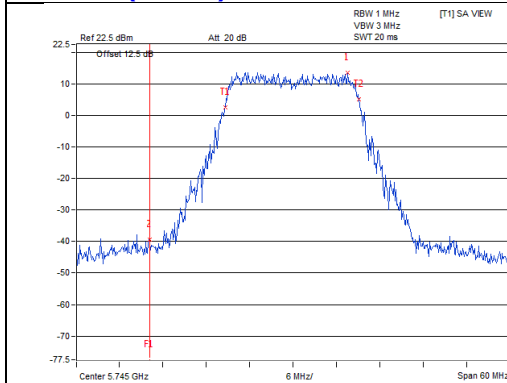
802.11ac (VHT20)_Chain 4 / CH149
