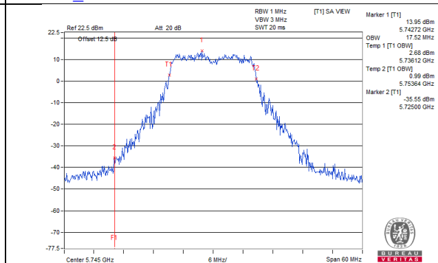
802.11a_Chain 7 / CH149
