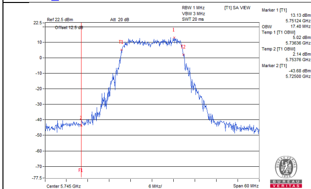
802.11a_Chain 4 / CH149
