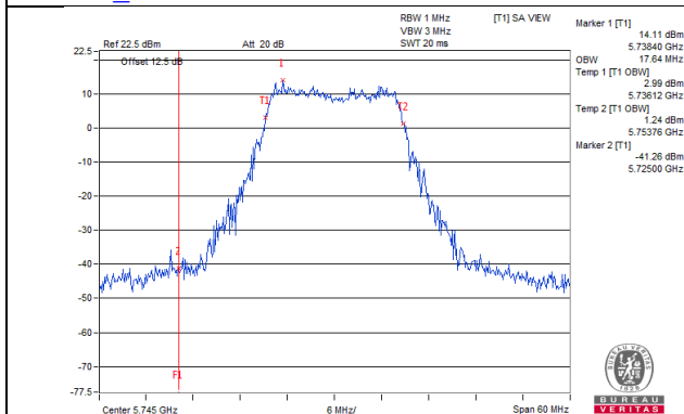
802.11a_Chain 6 / CH149
