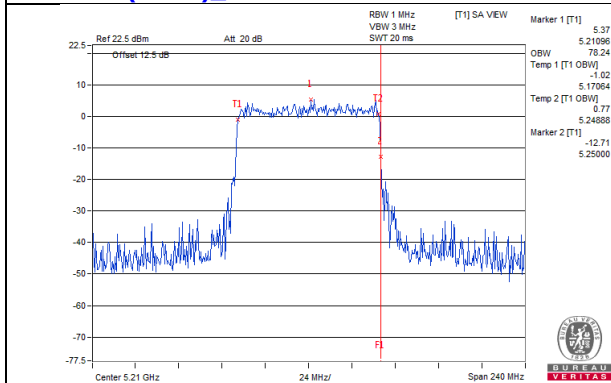
802.11ax (HE80)_Chain 4 / CH42
