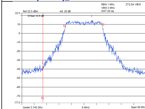
802.11ac (VHT20)_Chain 6 / CH149
