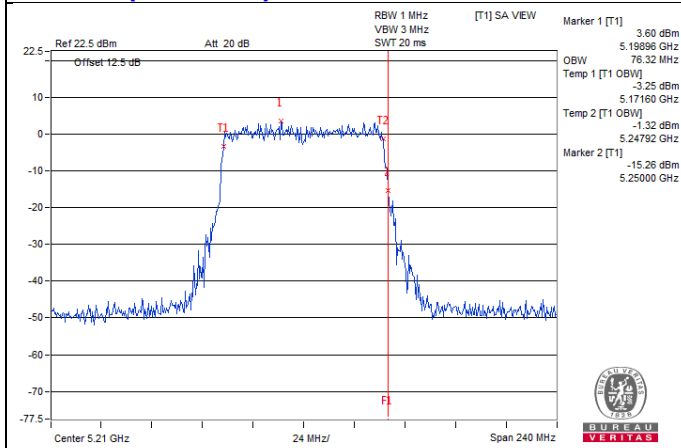
802.11ac (VHT80+80) / Chain 6 : CH42
