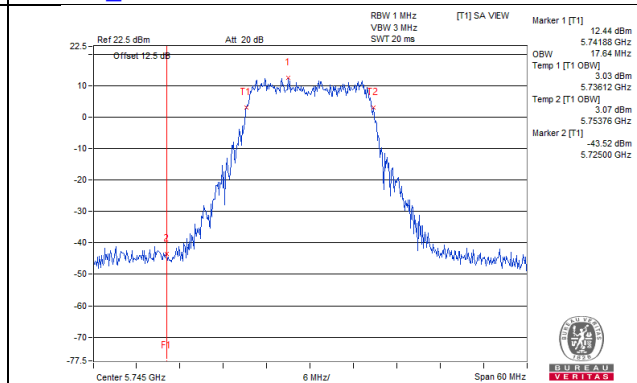
802.11a_Chain 5 / CH149
