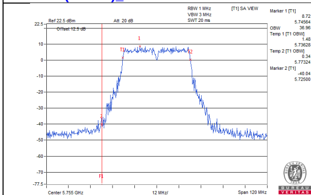
802.11ac (VHT40)_Chain 6 / CH151
