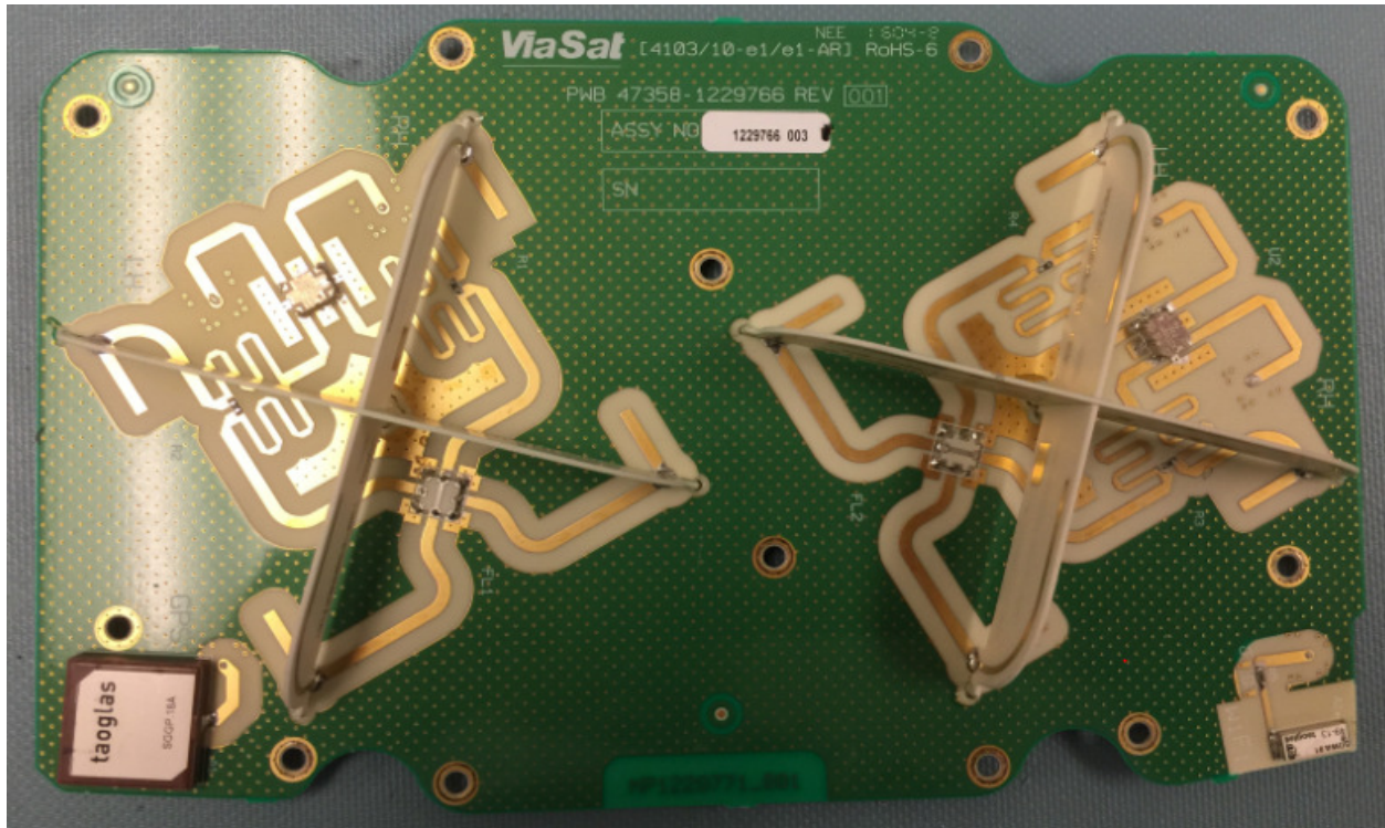
Antenna Board Bottom View
