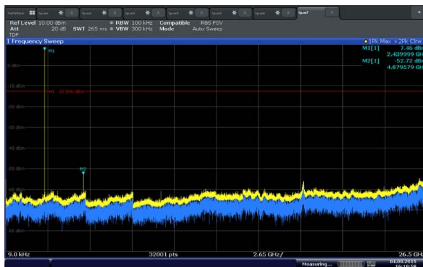
Mid Channel (GFSK)
