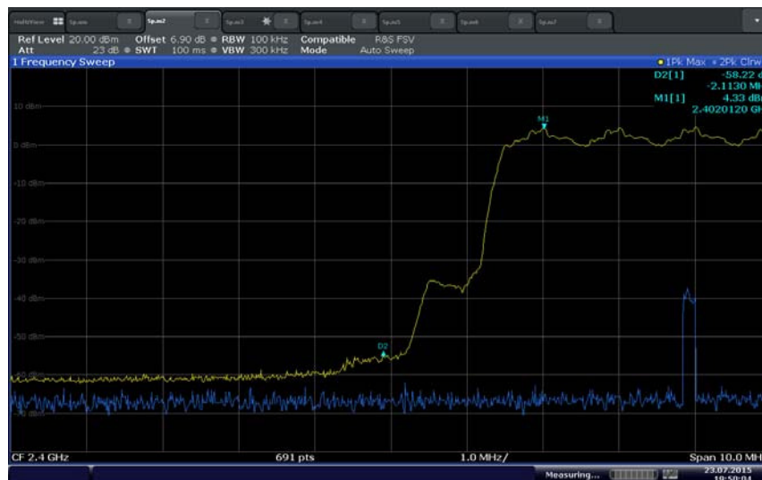
Hopping lower bandedge ( \pi/4 -DQPSK)
