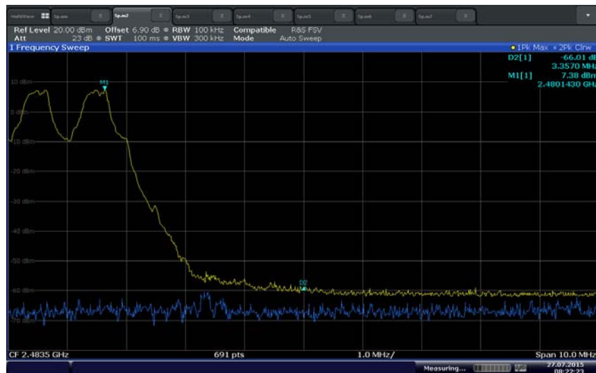
Hopping upper bandedge (GFSK)
