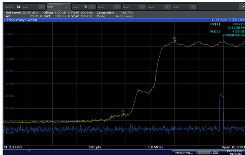
Hopping lower bandedge ( \pi/4 -DQPSK)
