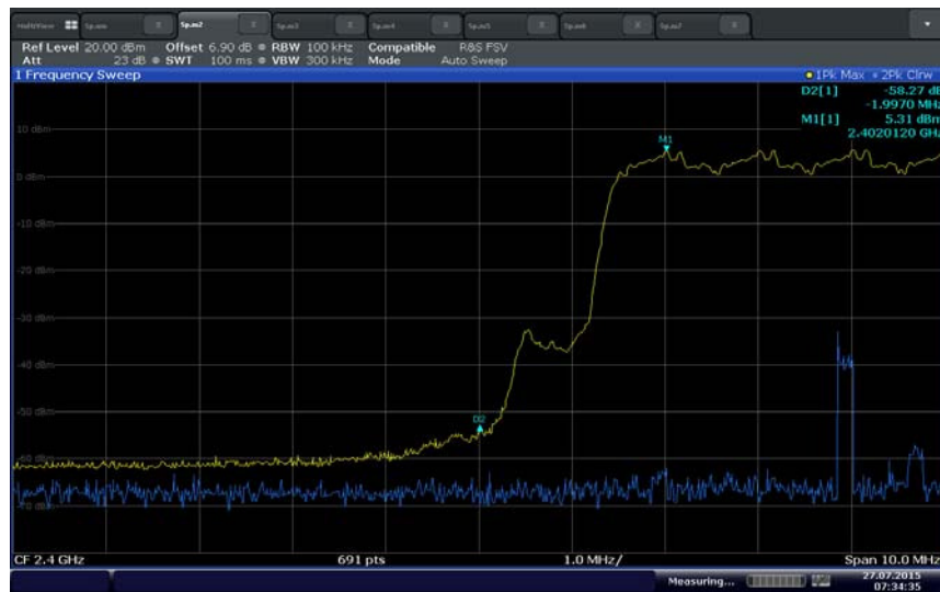
Hopping lower bandedge (8DPSK)
