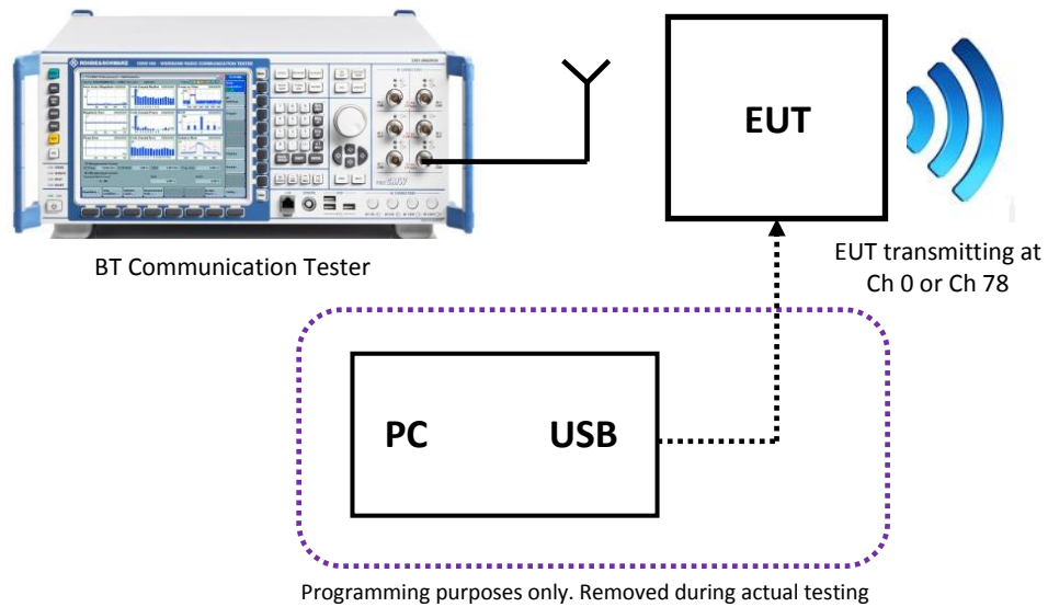
Test configuration used for radiated emissions testing
