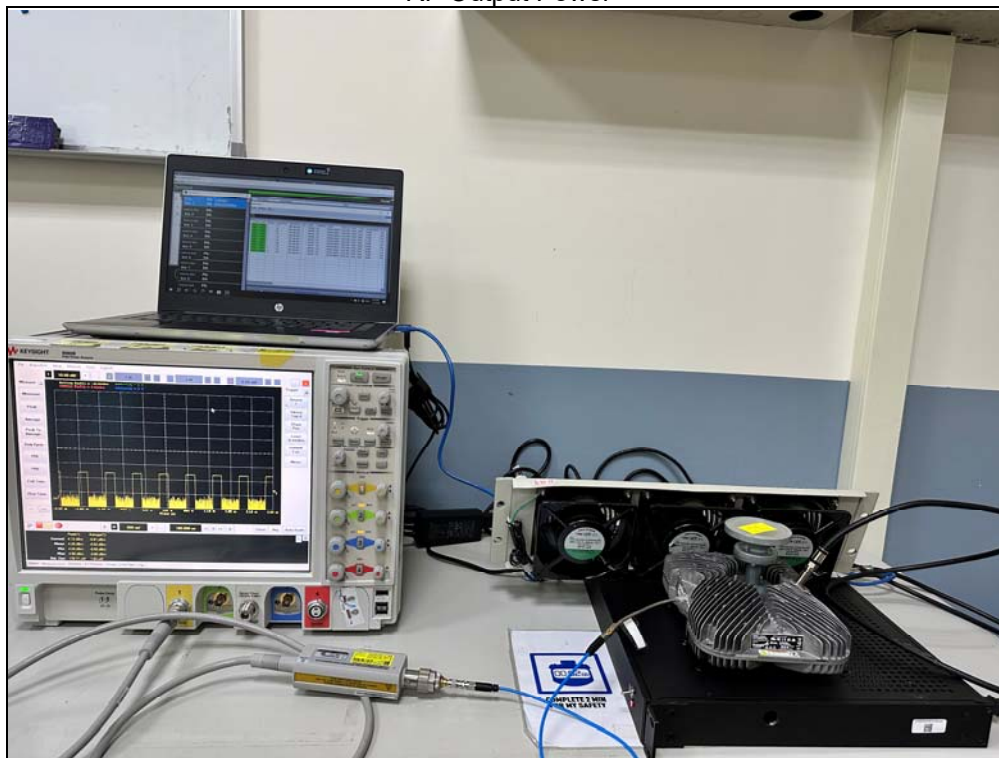
Conducted Measurement
