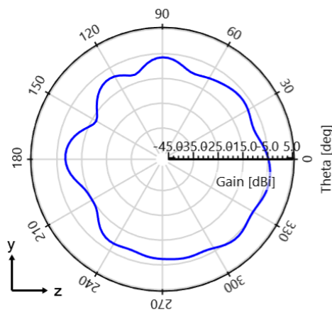
Gain (Total) - \phi = 90^\circ - 2440 MHz [Plane YZ]
