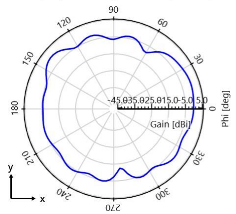
Gain (Total) - \theta = 90^\circ - 2440 MHz [Plane XY]
