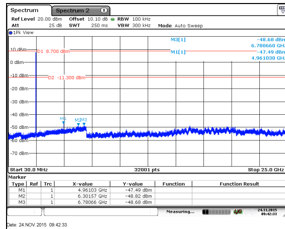
Figure 7.5.1.2-4: 30 MHz – 25 GHz – CH26
