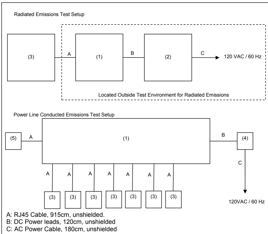
Figure 6-1: Test Setup Block Diagram
