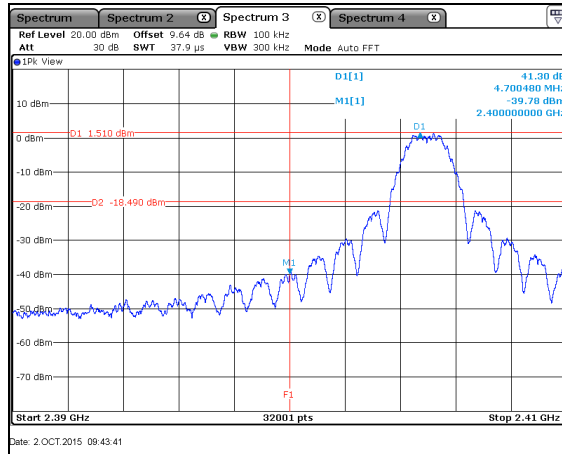
Figure 7.5.1.2-5: Lower Band-edge – CH11
