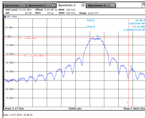
Figure 7.5.1.2-7: Upper Band-edge – CH26
