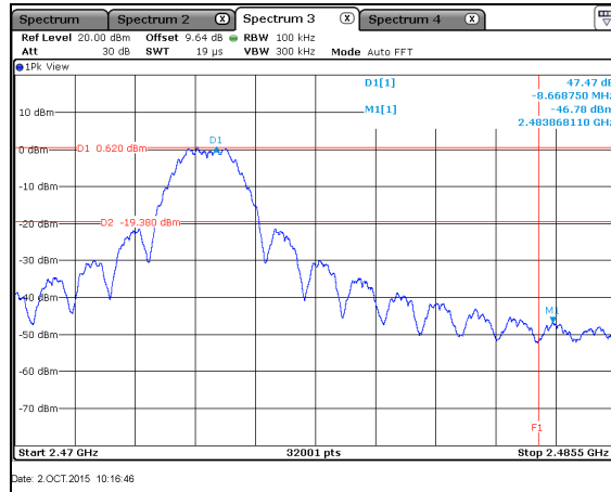
Figure 7.5.1.2-6: Upper Band-edge – CH25
