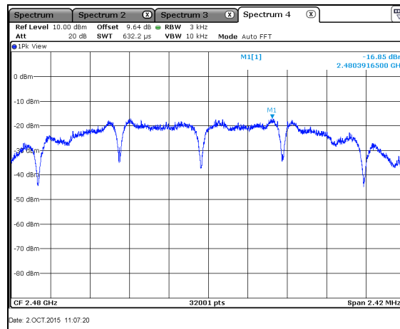
Figure 7.6.2-3: PSD Plot – CH26
