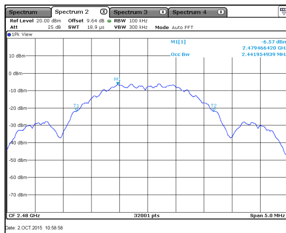
Figure 7.3.2-6: 99% Bandwidth Plot – CH 26
