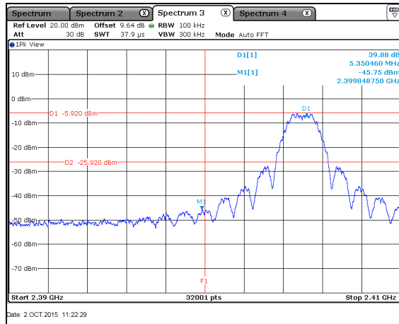
Figure 7.5.1.2-4: Lower Band-edge – CH11
