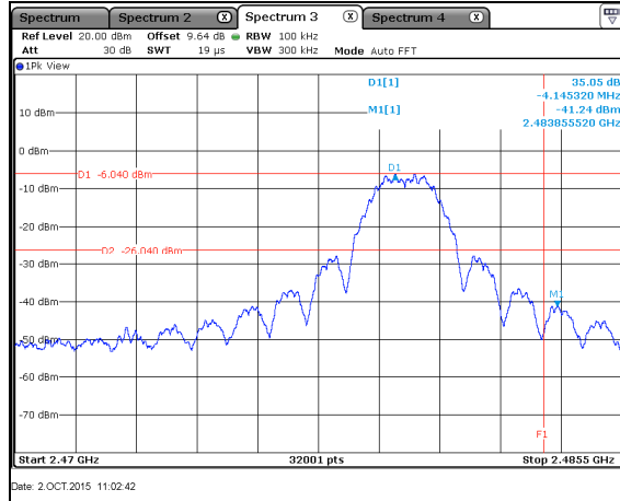
Figure 7.5.1.2-5: Upper Band-edge – CH26
