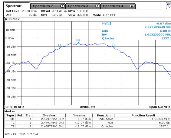
Figure 7.3.2-3: 6dB Bandwidth Plot – CH 26
