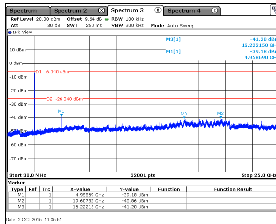
Figure 7.5.1.2-3: 30 MHz – 25 GHz – CH26
