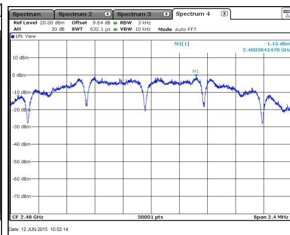
Figure 7.6.2-4: PSD Plot – HCH – CH 26
