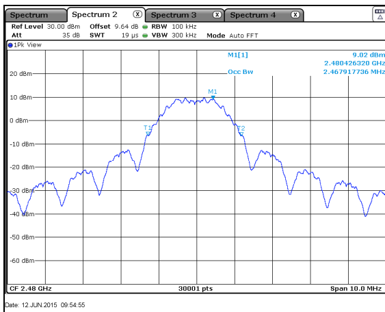
Figure 7.3.2-8: 99% Bandwidth Plot – HCH – CH 26
