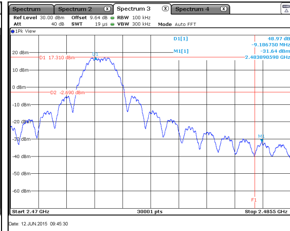
Figure 7.5.1.2-6: Upper Band-edge - HCH - CH 25
