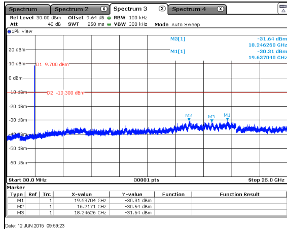
Figure 7.5.1.2-4: 30 MHz – 25 GHz – HCH – CH 26
