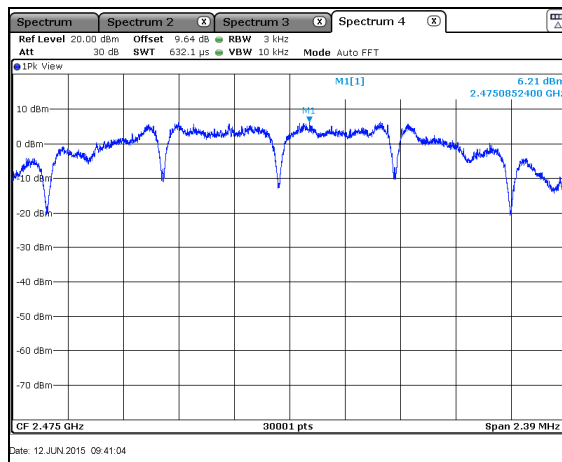
Figure 7.6.2-3: PSD Plot – HCH – CH 25
