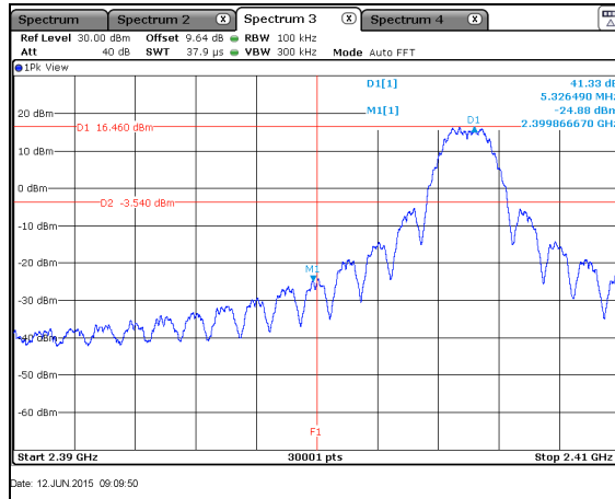
Figure 7.5.1.2-5: Lower Band-edge - LCH
