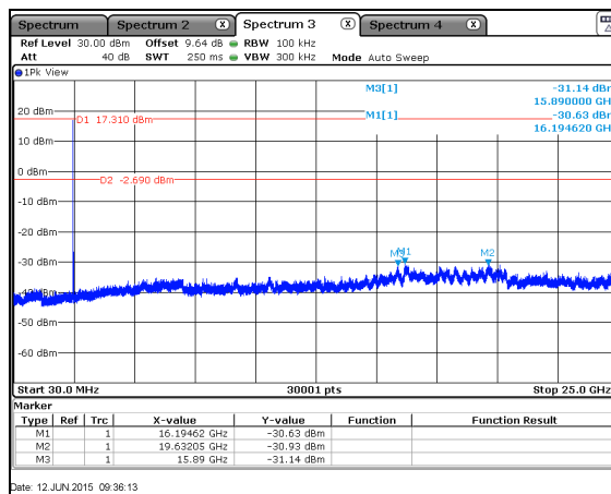
Figure 7.5.1.2-3: 30 MHz – 25 GHz – HCH – CH 25
