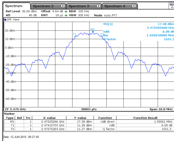
Figure 7.3.2-3: 6dB Bandwidth Plot – HCH – CH 25
