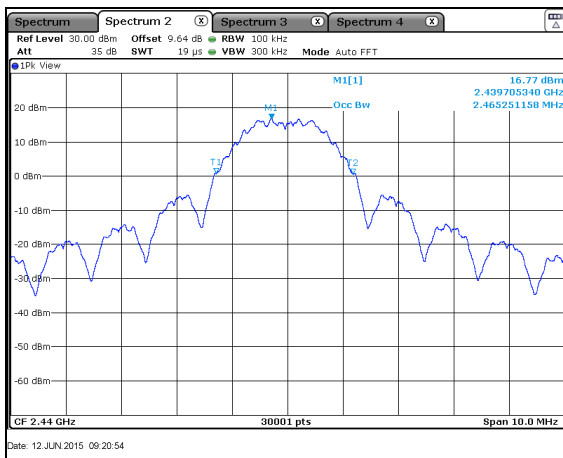
Figure 7.3.2-6: 99% Bandwidth Plot – MCH
