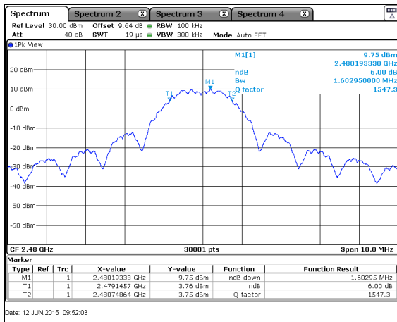
Figure 7.3.2-4: 6dB Bandwidth Plot – HCH – CH 26
