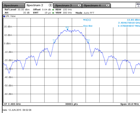
Figure 7.3.2-5: 99% Bandwidth Plot – LCH
