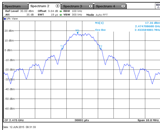
Figure 7.3.2-7: 99% Bandwidth Plot – HCH – CH 25
