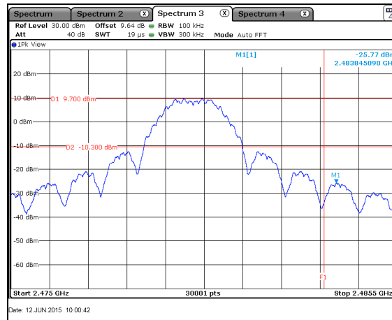
Figure 7.5.1.2-7: Upper Band-edge - HCH - CH 26
