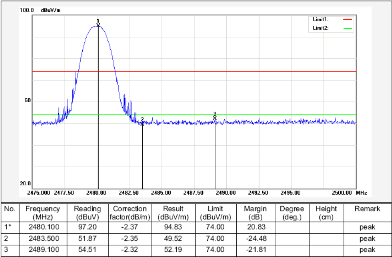
TEST PLOT OF BAND EDGE FOR HIGH CHANNEL –Horizontal
