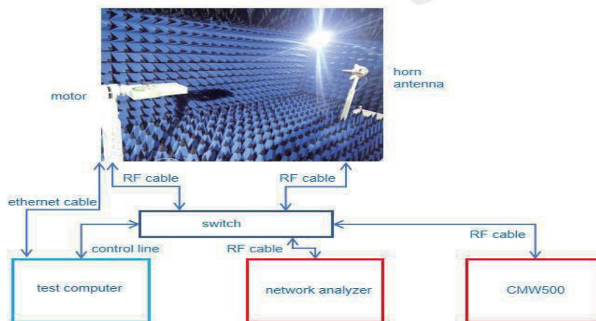
Antenna chamber structure
