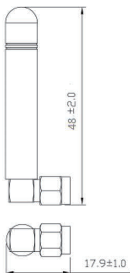
Antenna chamber structure
