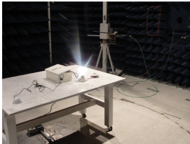
Radiated Emissions Setup, 1GHz - 10GHz
