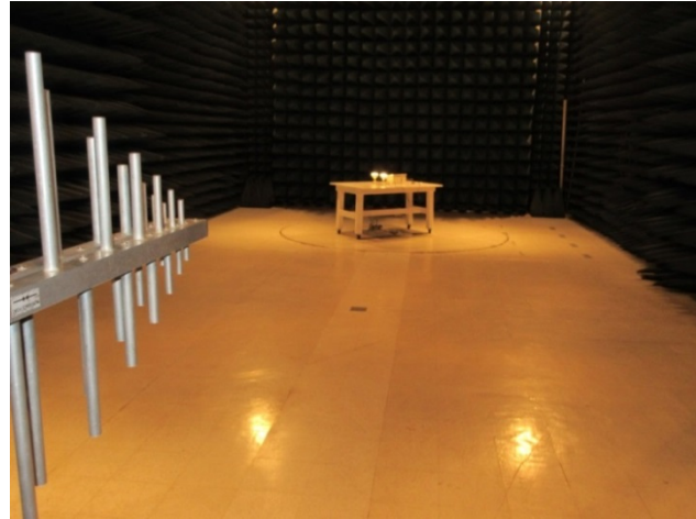
Radiated Emissions Setup, 200-1000 MHz
