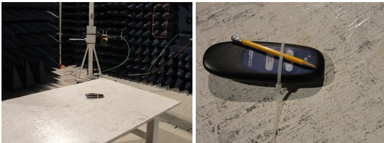
Operating Frequency per 47CFR15.249c Test Setup
