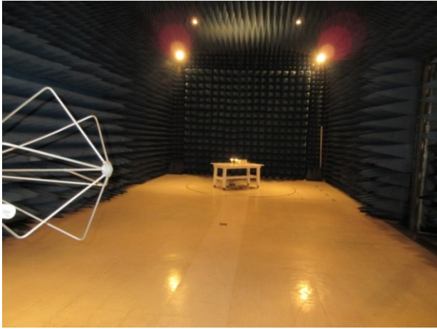
Radiated Emissions Setup, 30-200 MHz
