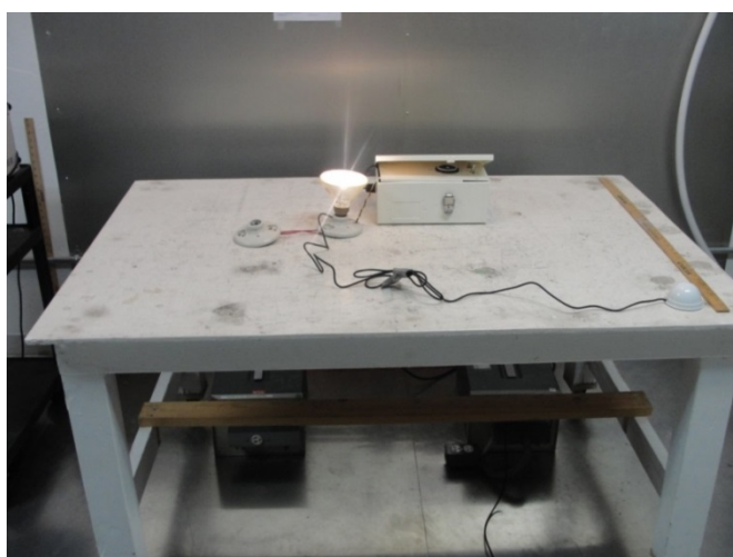
WPC Conducted Emissions Setup
