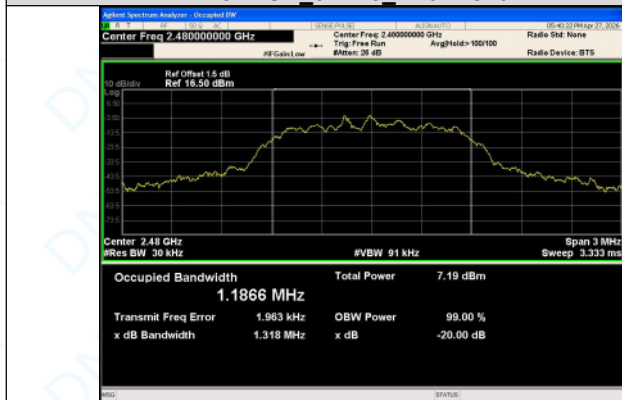
8DPSK_3-DH5_Channel 78
