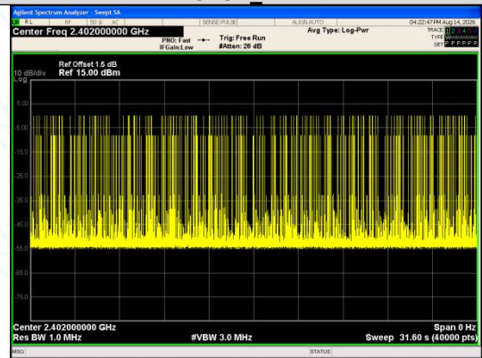
Number of Pulses in 31.6 seconds GFSK_DH3
