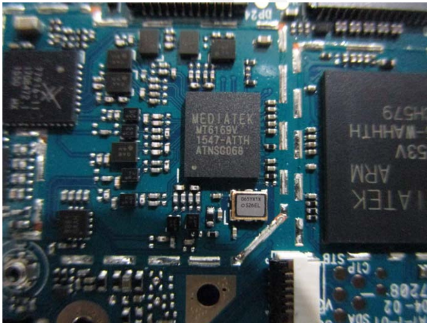
EUT –Chipset 3 View
