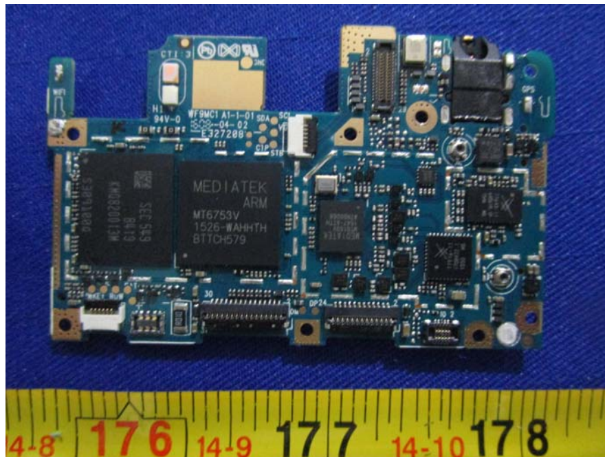
EUT –Main PCB Top Unshielded View
