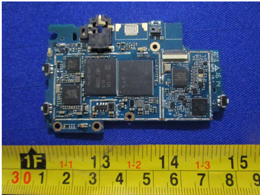
EUT –PCB1 Uncover Back View
