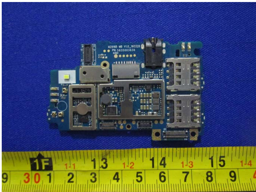
EUT –PCB1 Uncover Top View
