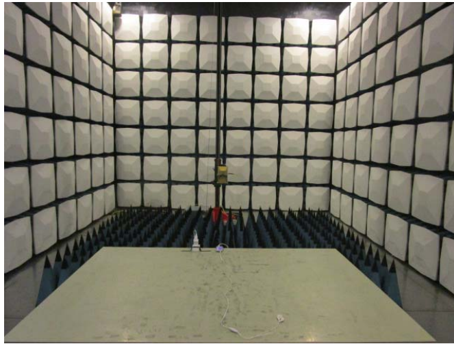
Radiated Emission - Front View (Above 1GHz)
