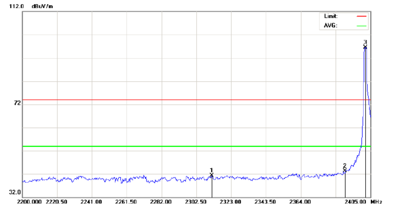
TEST PLOT OF BAND EDGE FOR LOW CHANNEL (3Mbps)-Horizontal
