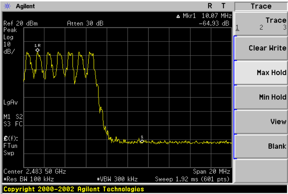
High band edge with hopping on (GFSK)
