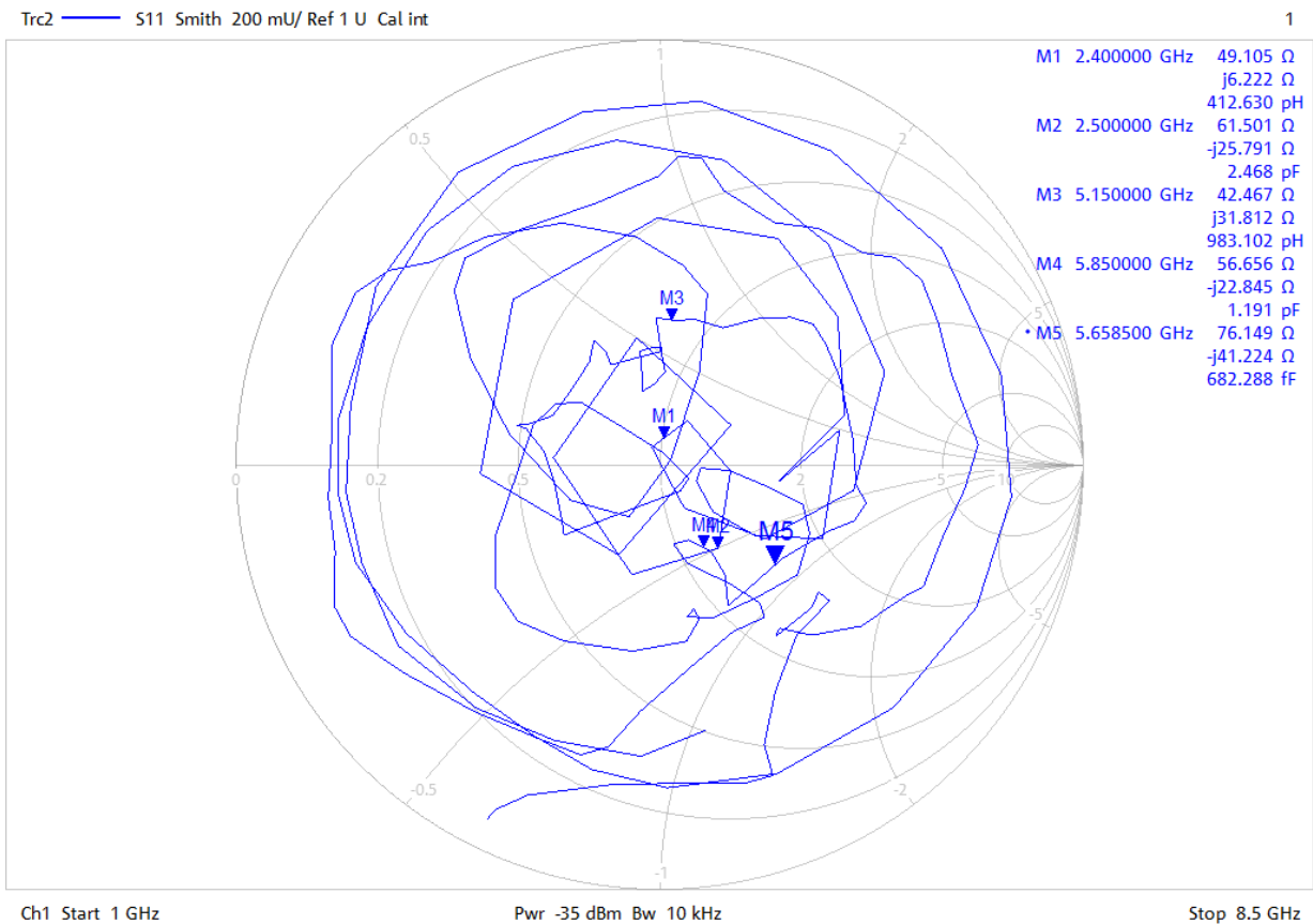
Smith Circle diagram
