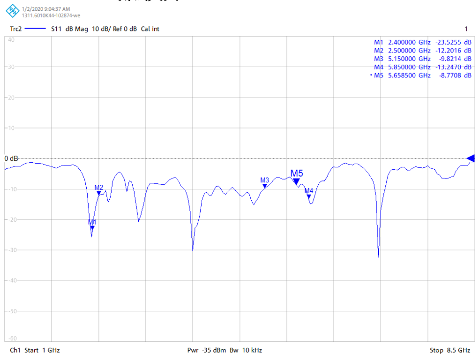
S11 Graph
