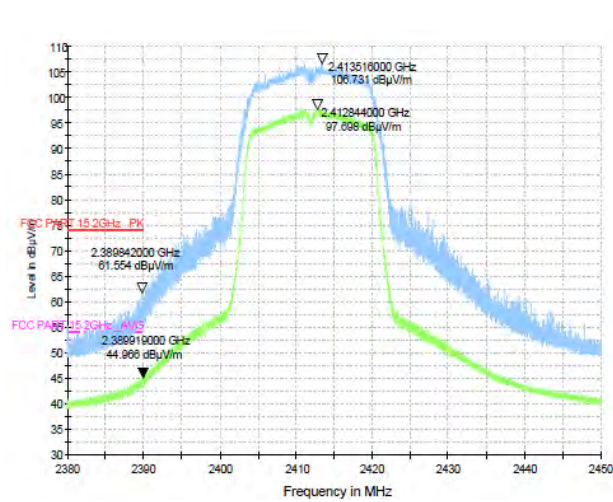
Test Mode: IEEE 802.11g-Low
