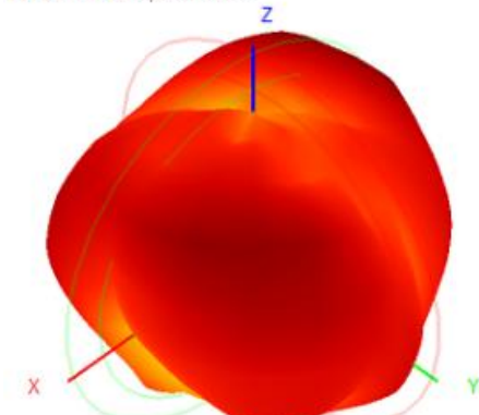
5850.0MHz H+V, Eff: 59.9%
