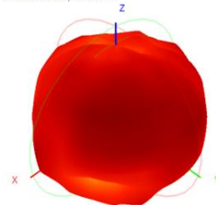
5850.0MHz H+V, Eff: 59.9%
