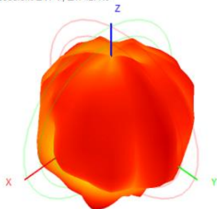
5850.0MHz H+V, Eff: 42.4%
