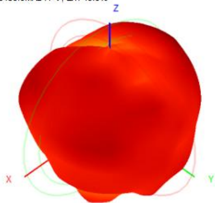
2450.0MHz H+V, Eff: 49.0%
