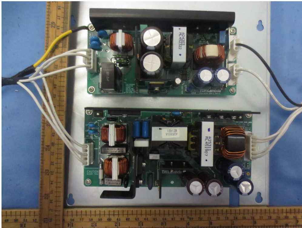
Ancillary equipment (power supply)
