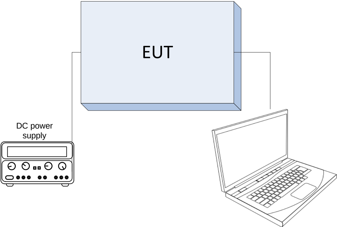
Figure 3.5-1: Setup diagram
