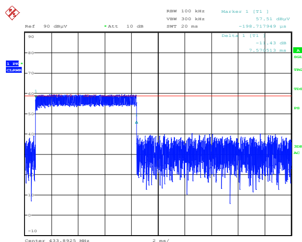
Figure 8.1-5: TDM LRFQ service mode (7.57 ms)
