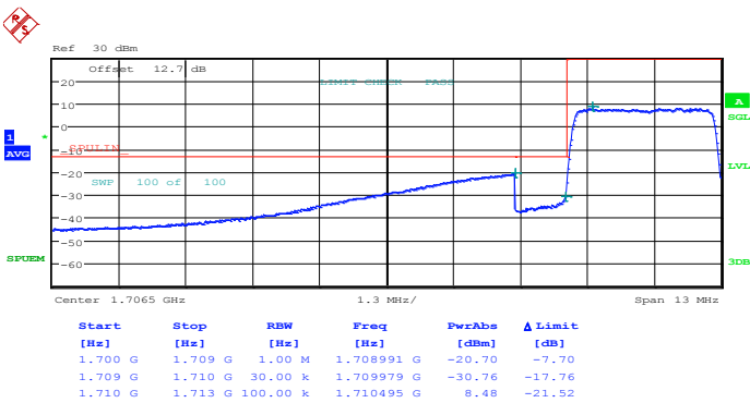
Lower Band Edge Plot for 16QAM-RB Size 15, RB Offset 0
