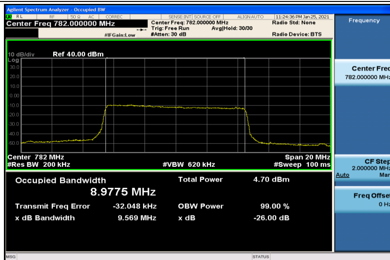
Band13-10MHz-16QAM-23230-50RB#0-8.9806
