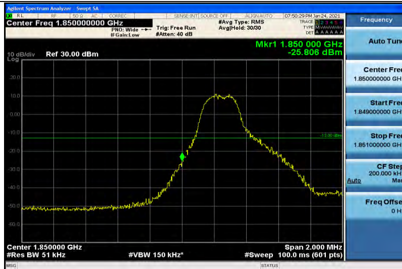
Band2-3MHz-16QAM-18615-1RB#14
