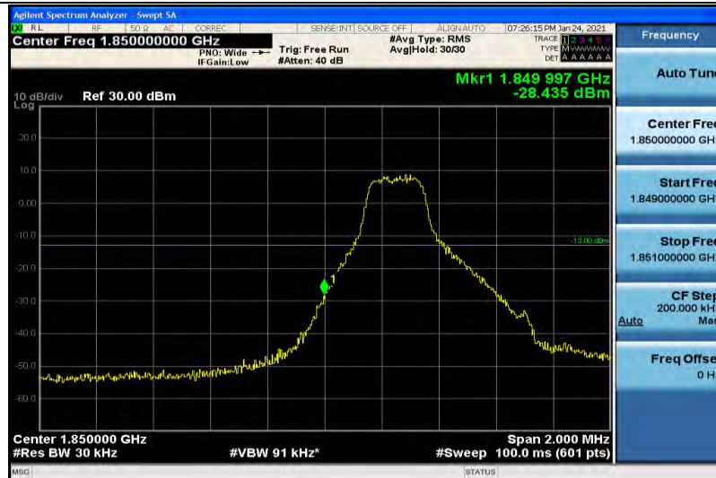
Band2-1.4MHz-16QAM-18607-1RB#5
