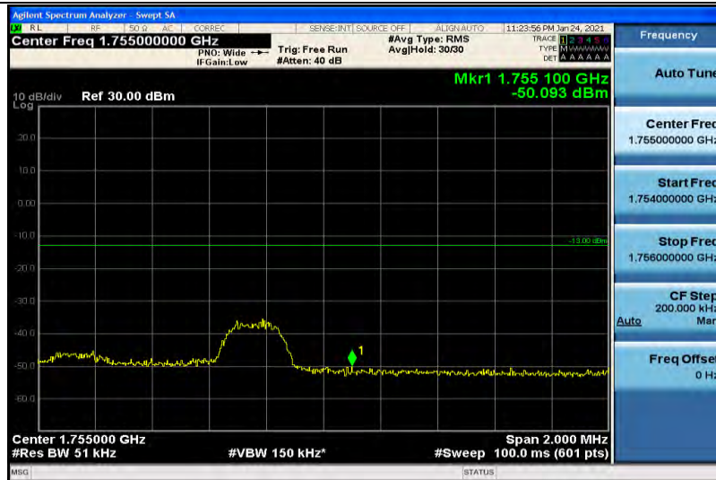
Band4-3MHz-16QAM-20385-1RB#14
