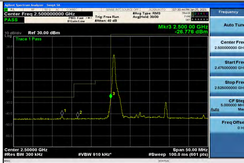
Band7-15MHz-16QAM-20825-1RB#74
