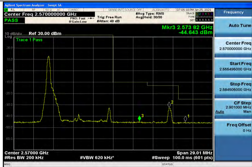
Band7-10MHz-16QAM-21400-1RB#49
