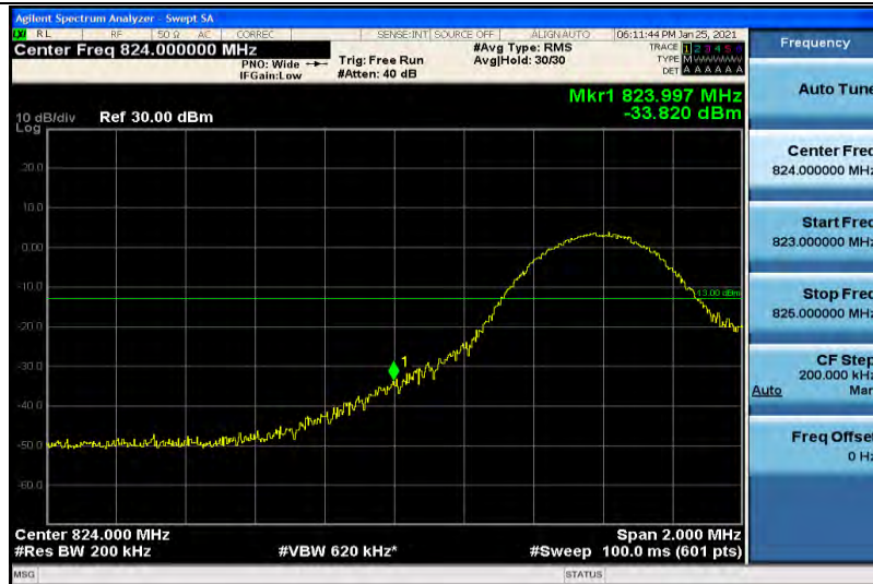
Band5-10MHz-16QAM-20450-1RB#49
