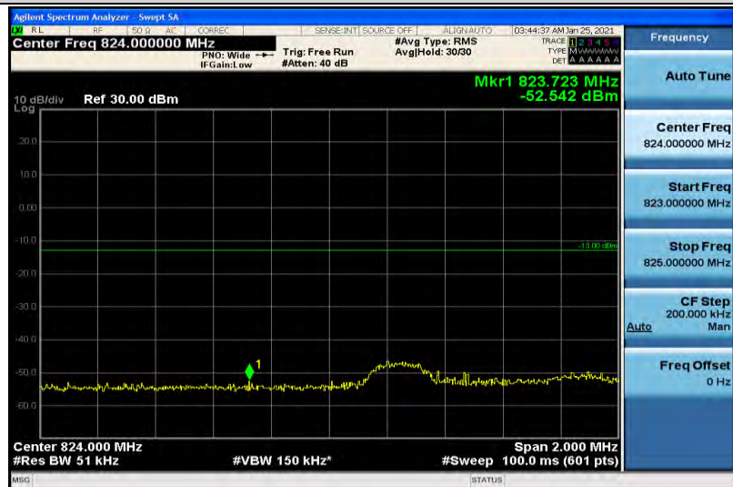
Band5-3MHz-QPSK-20415-15RB#0
