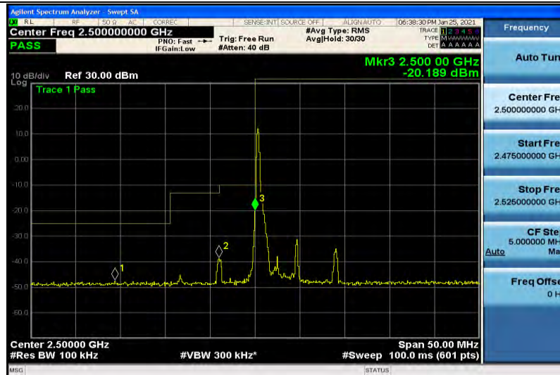
Band7-5MHz-QPSK-20775-1RB#24
