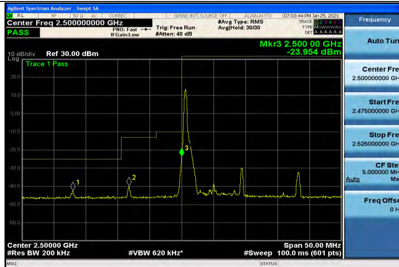
Band7-10MHz-QPSK-20800-1RB#49
