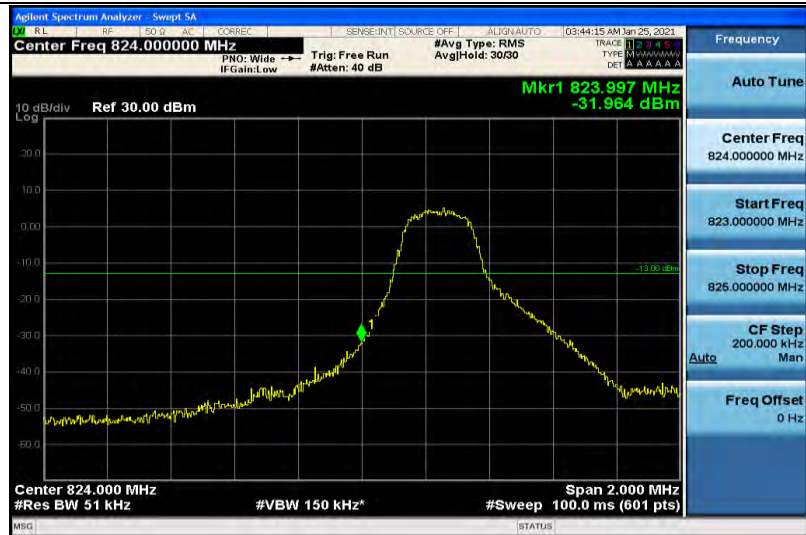
Band5-3MHz-QPSK-20415-1RB#14
