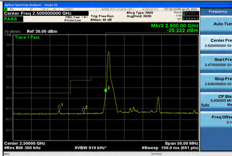
Band7-15MHz-QPSK-20825-1RB#74
