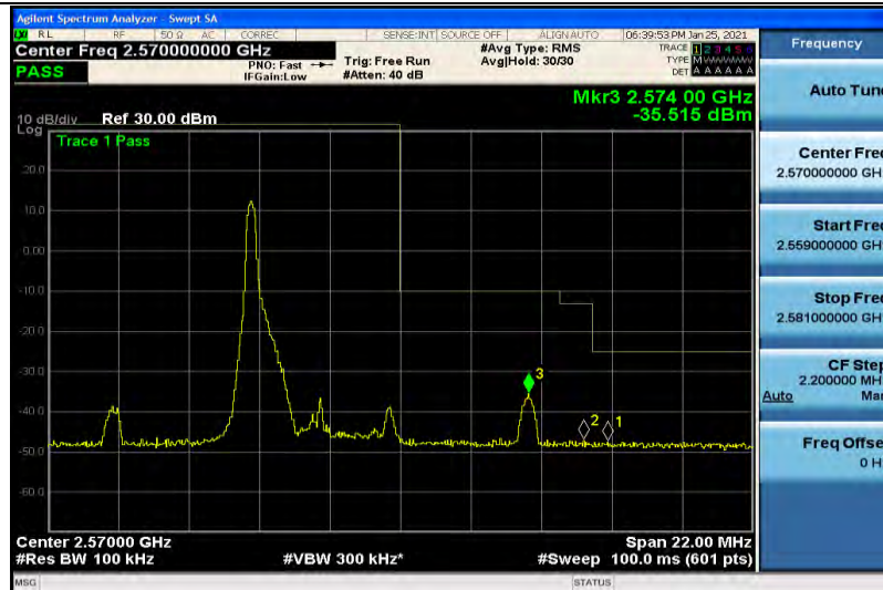
Band7-5MHz-QPSK-21425-1RB#24
