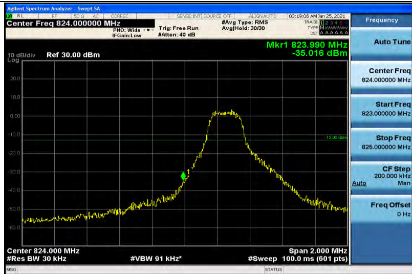
Band5-1.4MHz-QPSK-20407-1RB#5
