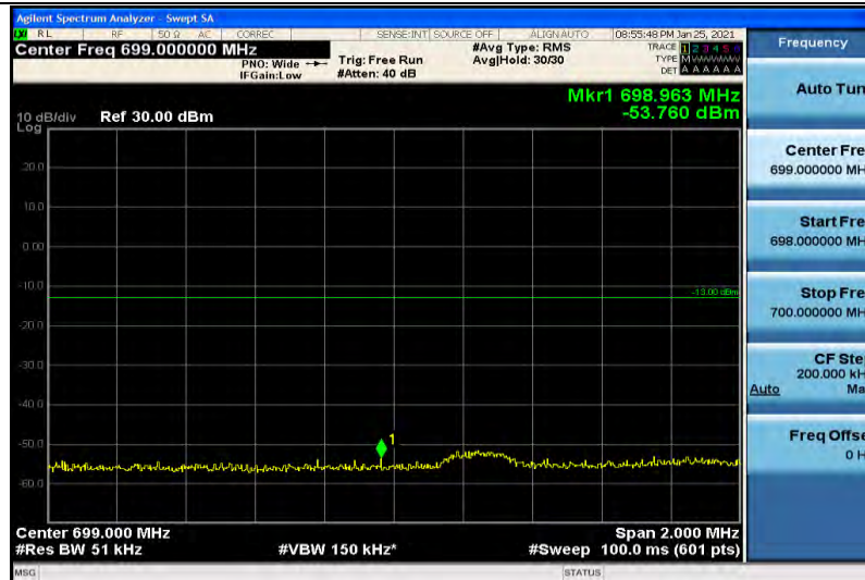
Band12-3MHz-16QAM-23025-1RB#0
