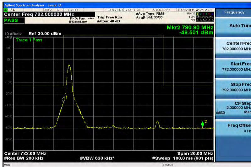
Band13-10MHz-16QAM-23230-1RB#49
