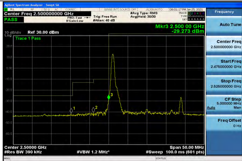
Band7-20MHz-16QAM-20850-1RB#99
