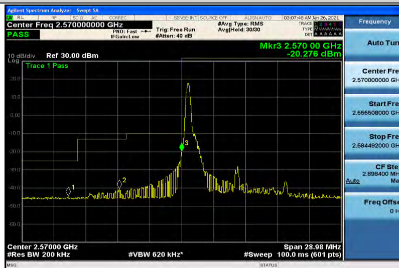
Band38-10MHz-16QAM-37800-50RB#0
