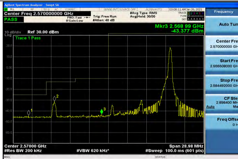
Band38-10MHz-16QAM-37800-1RB#0
