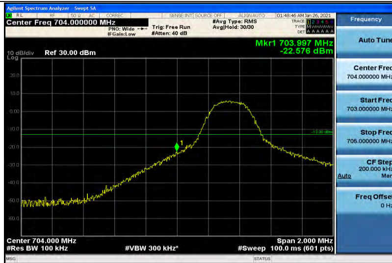
Band17-5MHz-QPSK-23755-1RB#24
