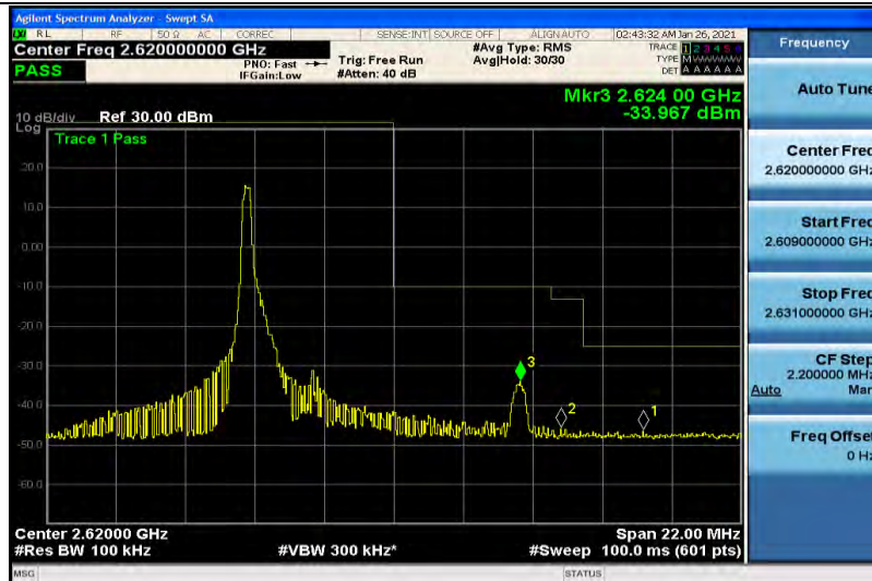
Band38-5MHz-QPSK-38225-1RB#24
