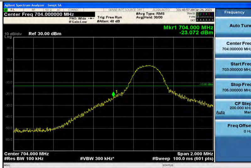
Band17-5MHz-16QAM-23755-1RB#24
