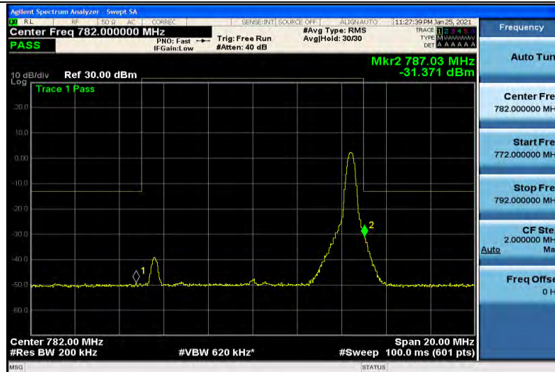
Band13-10MHz-QPSK-23230-1RB#0
