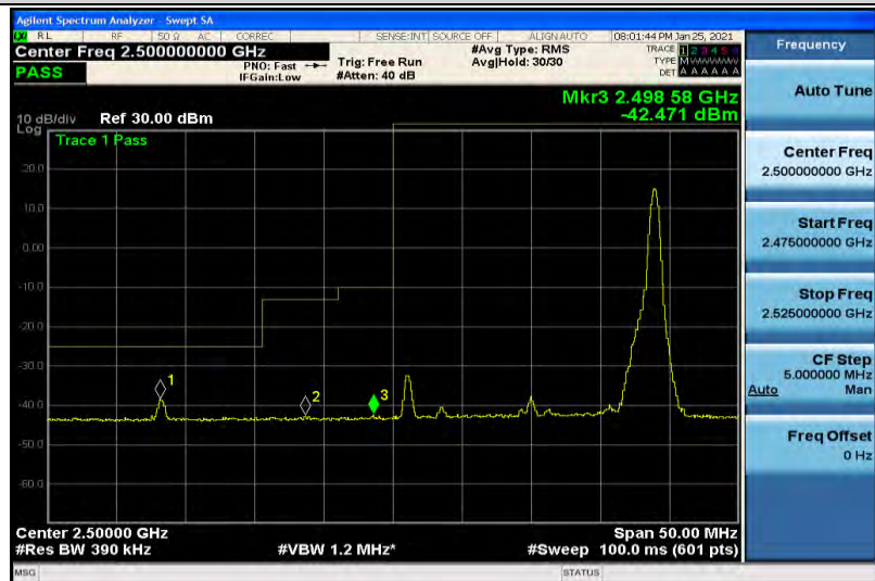
Band7-20MHz-16QAM-20850-100RB#0
