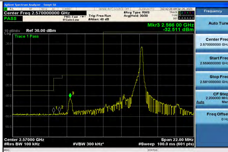
Band38-5MHz-QPSK-37775-1RB#0
