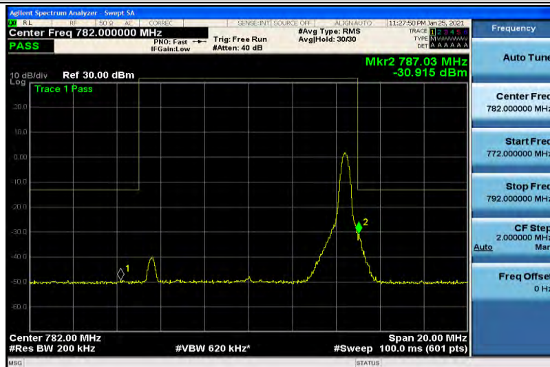
Band13-10MHz-16QAM-23230-50RB#0
