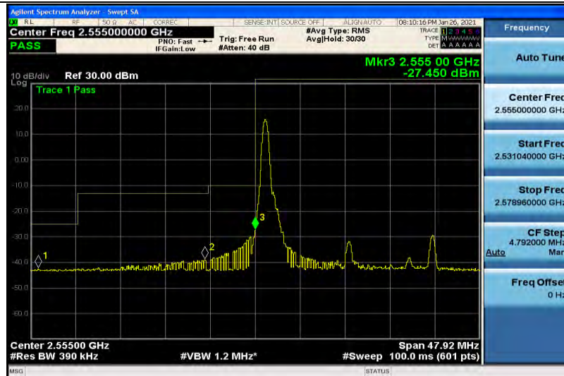
Band41-20MHz-QPSK-40340-1RB#99
