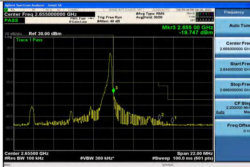
Band41-5MHz-QPSK-41215-1RB#0
