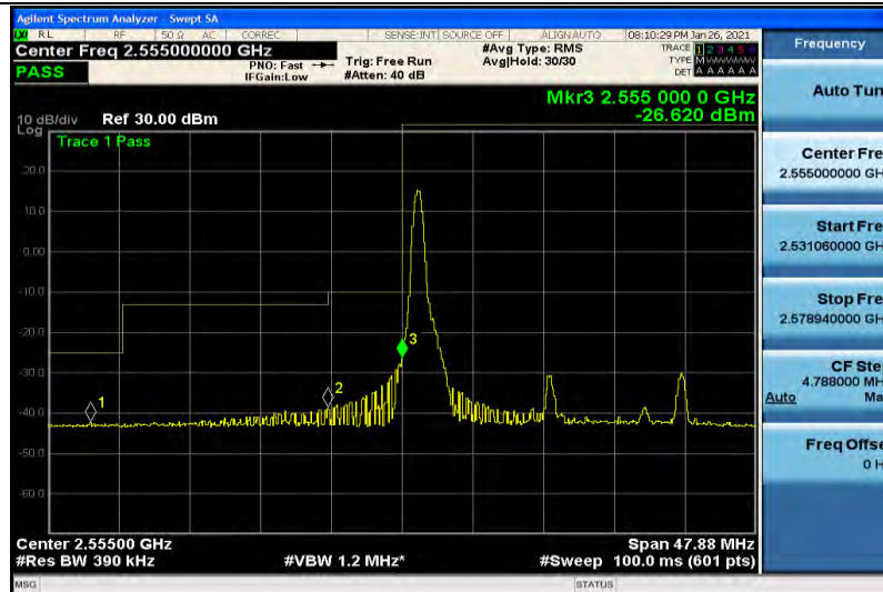
Band41-20MHz-16QAM-40340-1RB#99
