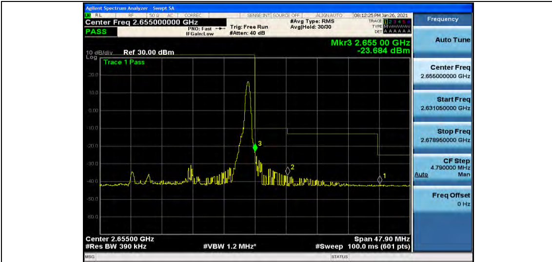
Band41-20MHz-16QAM-41140-1RB#0
