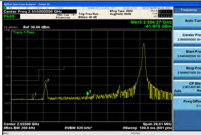
Band41-10MHz-16QAM-40290-1RB#0
