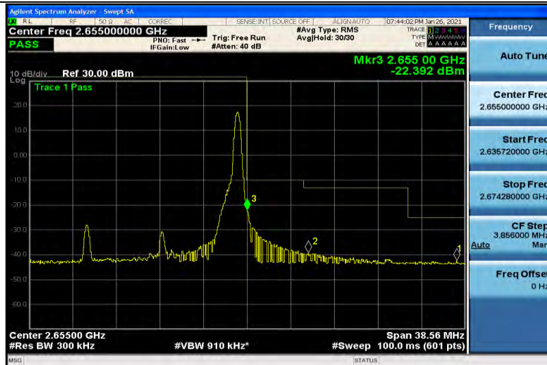
Band41-15MHz-QPSK-41165-1RB#0
