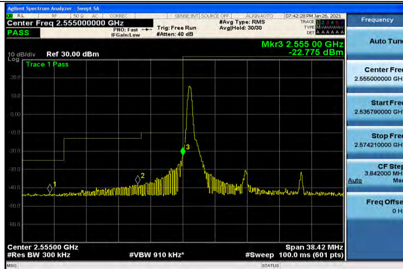
Band41-15MHz-16QAM-40315-1RB#74
