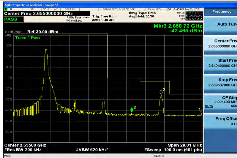
Band41-10MHz-QPSK-41190-1RB#49
