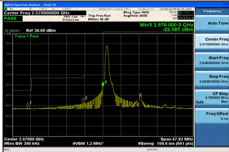
Band38-20MHz-16QAM-37850-1RB#99
