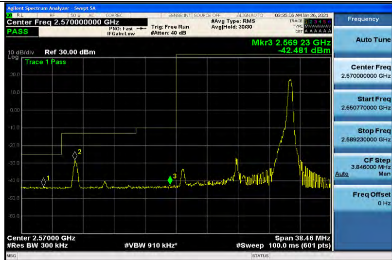
Band38-15MHz-16QAM-37825-1RB#0
