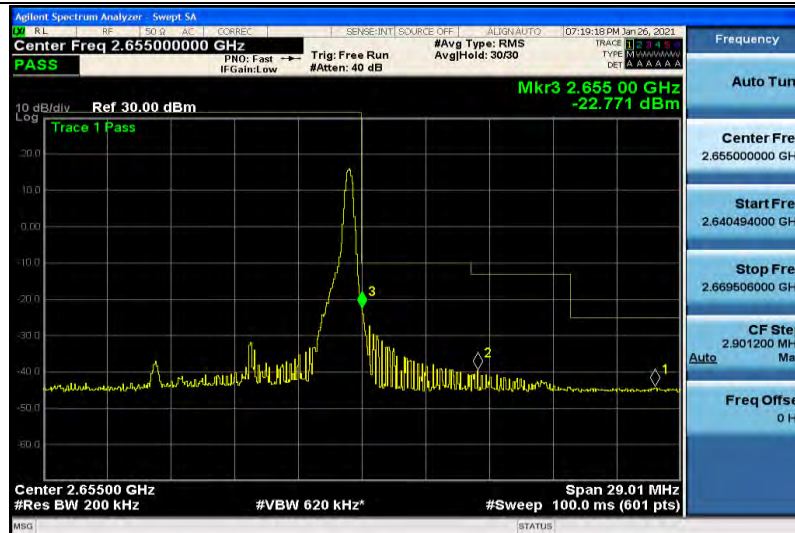
Band41-10MHz-16QAM-41190-1RB#0
