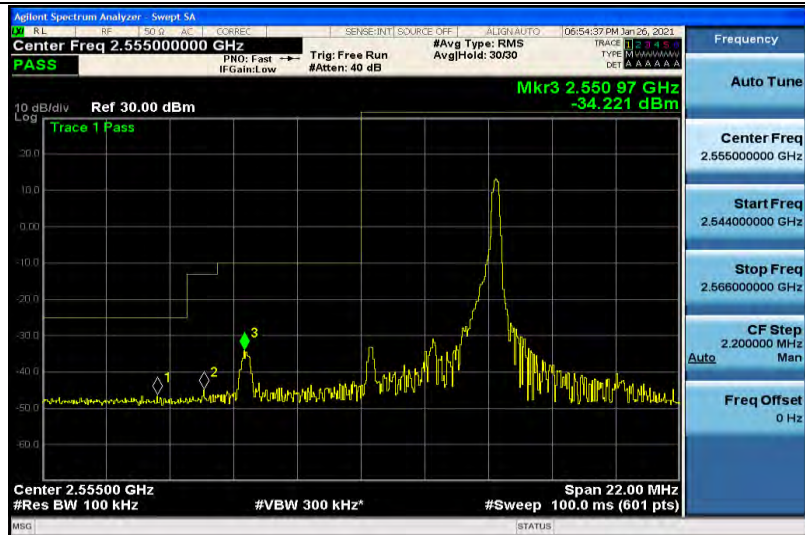
Band41-5MHz-16QAM-40265-1RB#0
