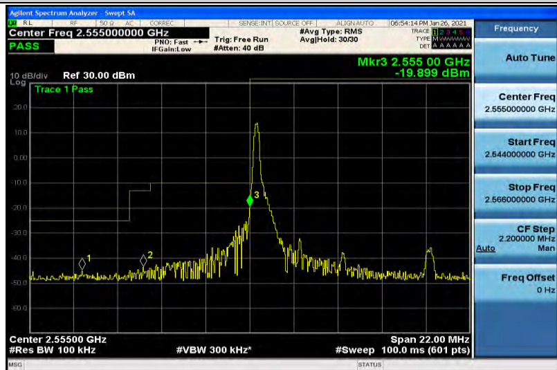
Band41-5MHz-16QAM-40265-25RB#0
