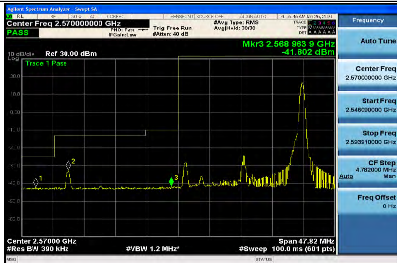
Band38-20MHz-16QAM-37850-100RB#0
