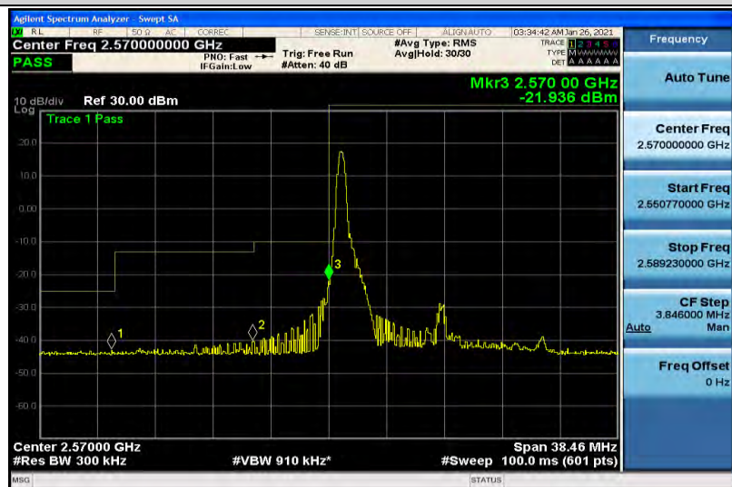
Band38-15MHz-16QAM-37825-75RB#0
