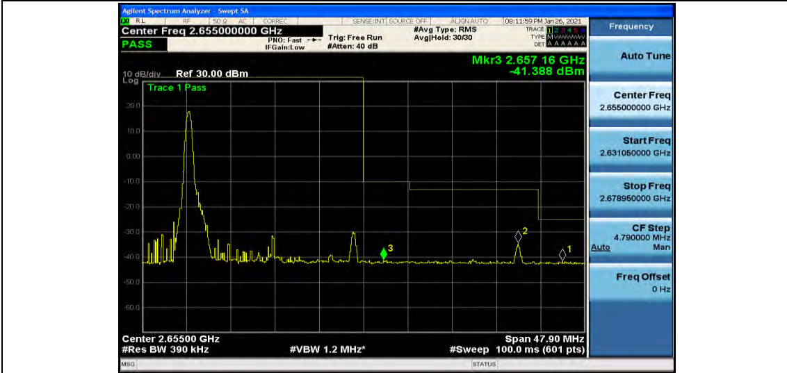
Band41-20MHz-16QAM-41140-100RB#0
