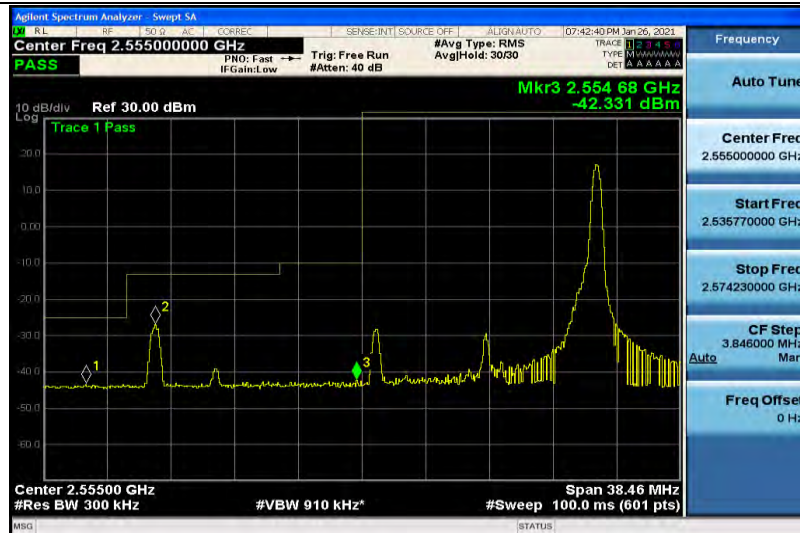
Band41-15MHz-QPSK-40315-1RB#0
