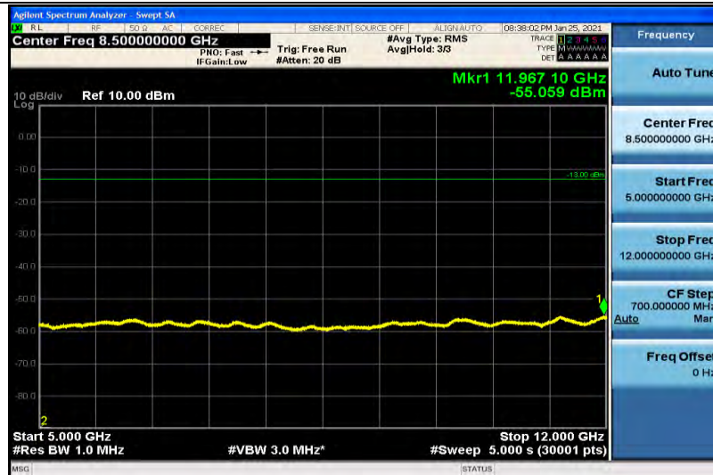
Band12-1.4MHz-16QAM-23095-1RB#0-Range4:12000~26500MHz
