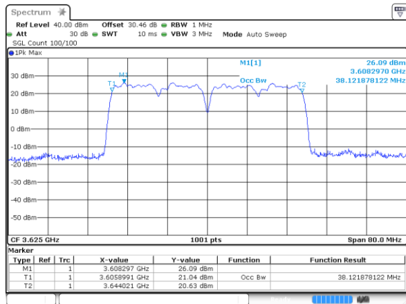
Middle Channel / 20MHz+20MHz
