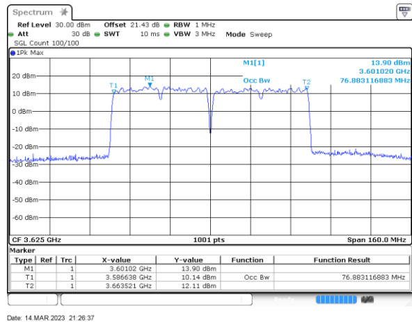
Middle Channel / 40MHz+40MHz
