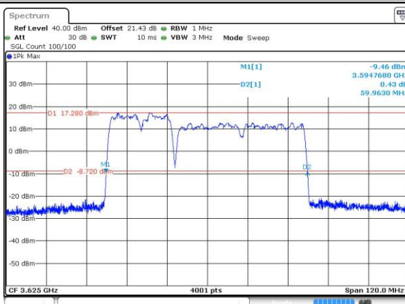
Middle Channel / 20MHz+40MHz
