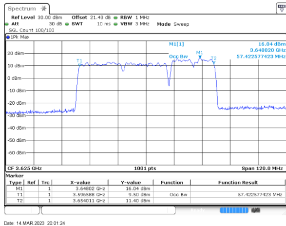
Middle Channel / 40MHz+20MHz
