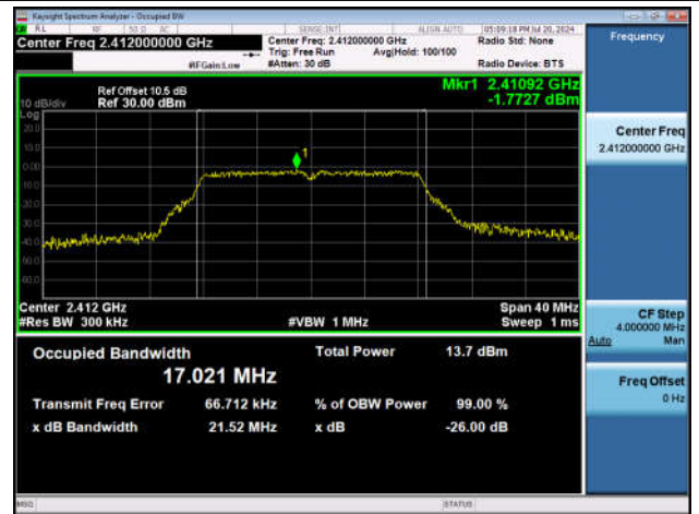
11G-Ant1-2412
