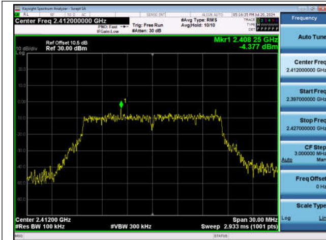
11G-Ant1-2412-0~Reference-PASS
