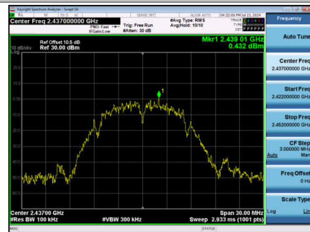
11B-Ant1-2437-0~Reference-PASS
