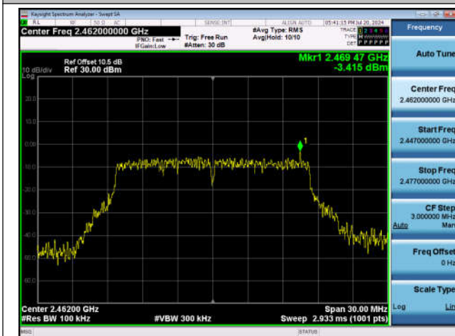
11G-Ant1-2462-0~Reference-PASS
