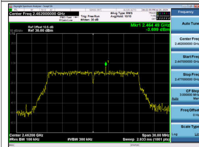
11N20SISO-Ant1-2462-0~Reference-PASS
