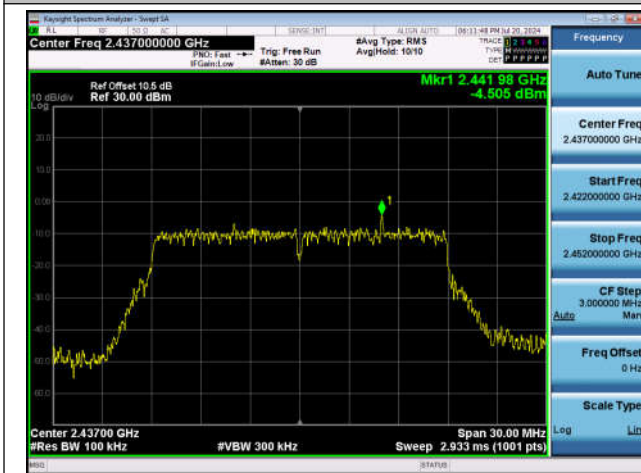
11N20SISO-Ant1-2437-0~Reference-PASS
