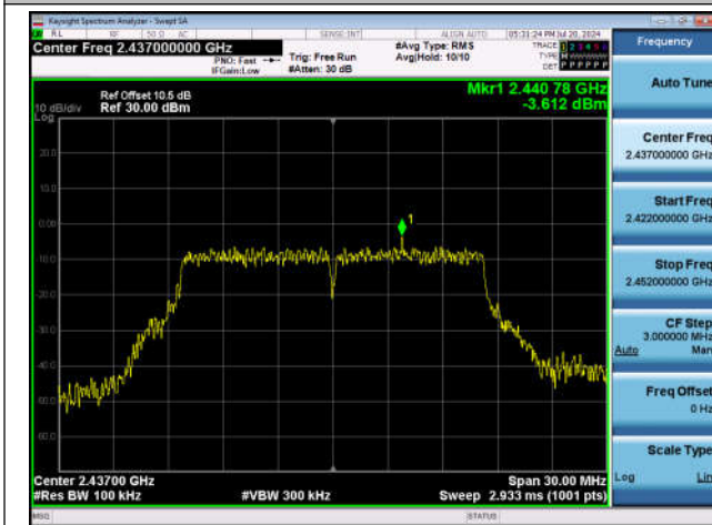
11G-Ant1-2437-0~Reference-PASS
