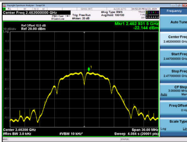
11B-Ant1-2462-PASS
