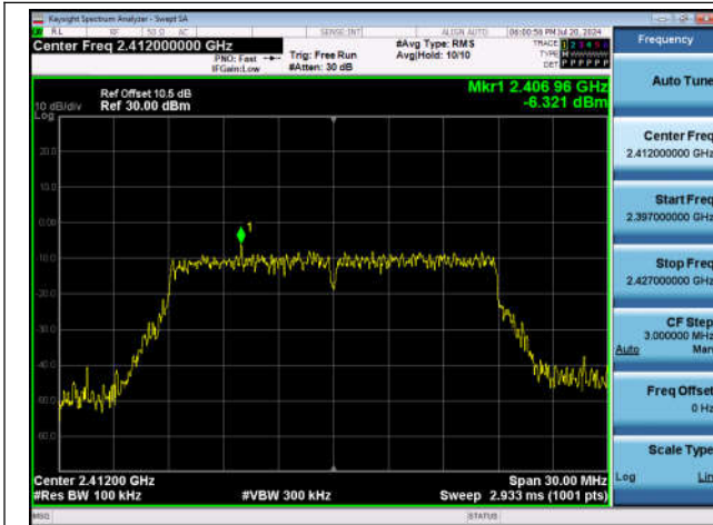
11N20SISO-Ant1-2412-0~Reference-PASS
