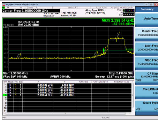
11G-Ant1-2412-PASS
