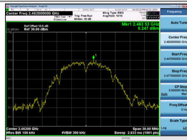
11B-Ant1-2462-0~Reference-PASS
