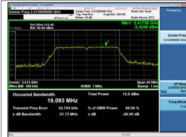
11N20SISO-Ant1-2412
