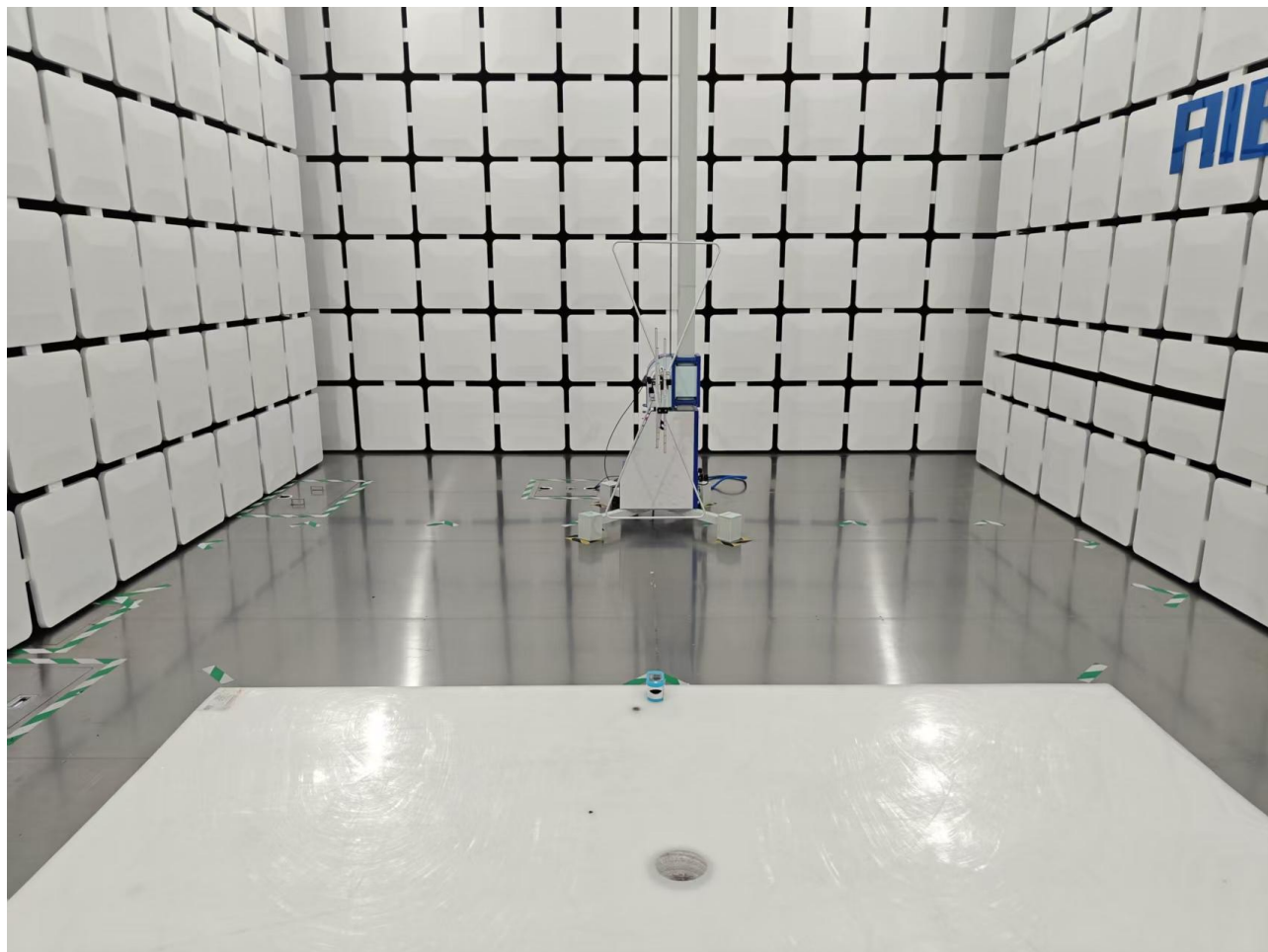
Radiated Emission Test View 1
