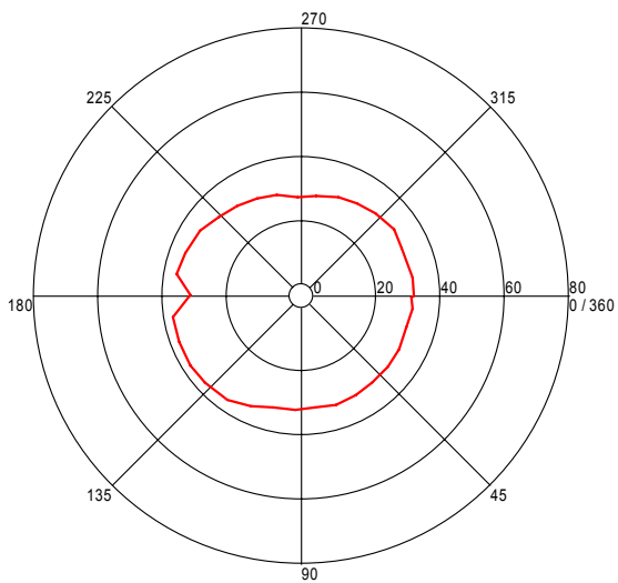
Turntable Plot ( 199.911422485 MHz )
