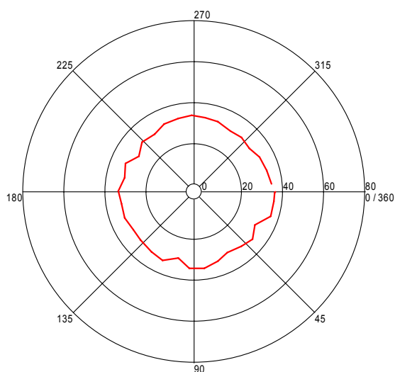
Turntable Plot ( 900.046092625 MHz )
