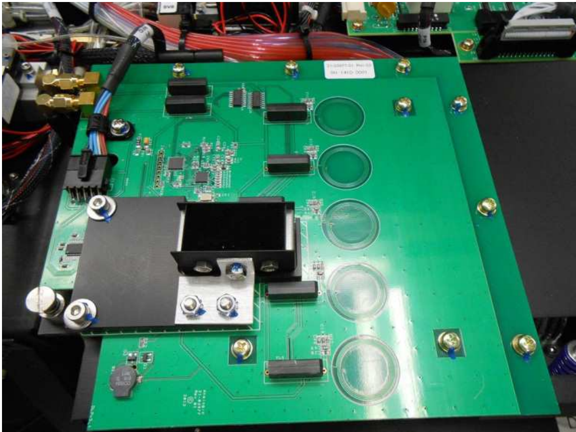
InstrumentInternal_RFIDReader
