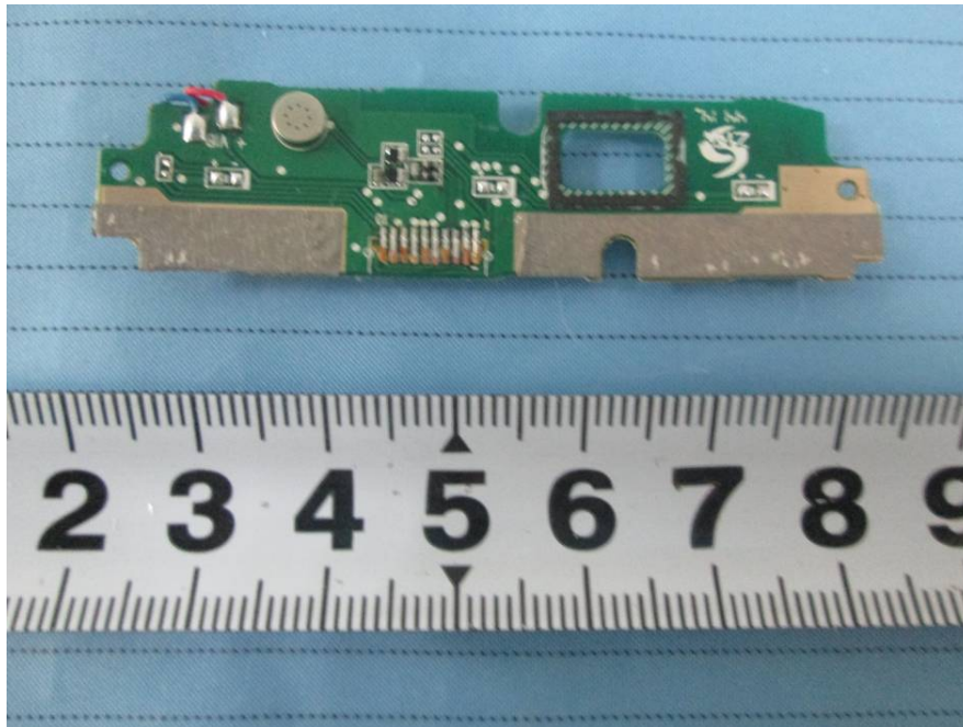
EUT –Connect PCB Board Bottom View
