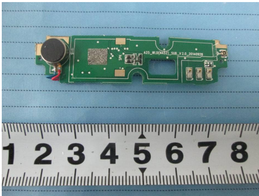
EUT – Connect PCB Board Top Shielding off View
