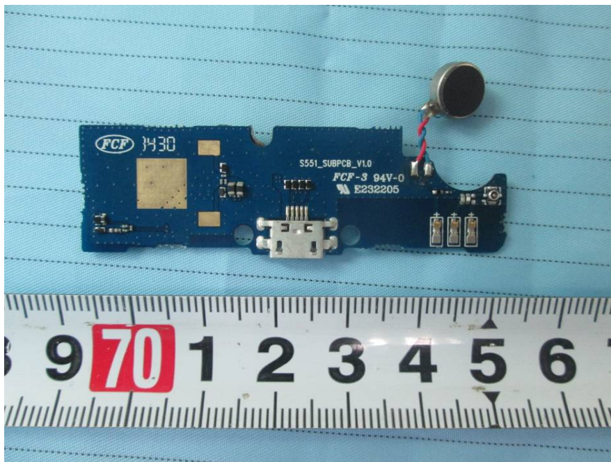
EUT – Connect PCB Top View
