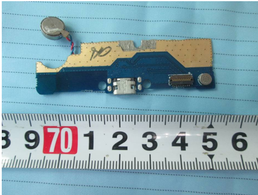
EUT –Connect PCB Bottom View
