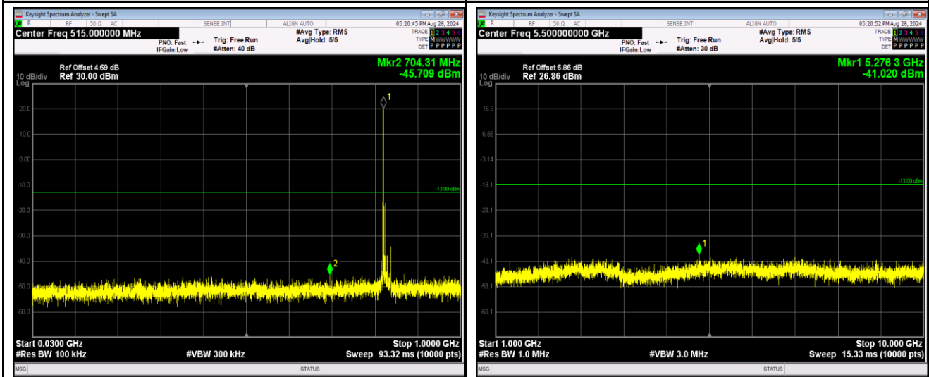
Band5-10MHz-64QAM-20525-1RB#0-Range1:30~1000MHz
