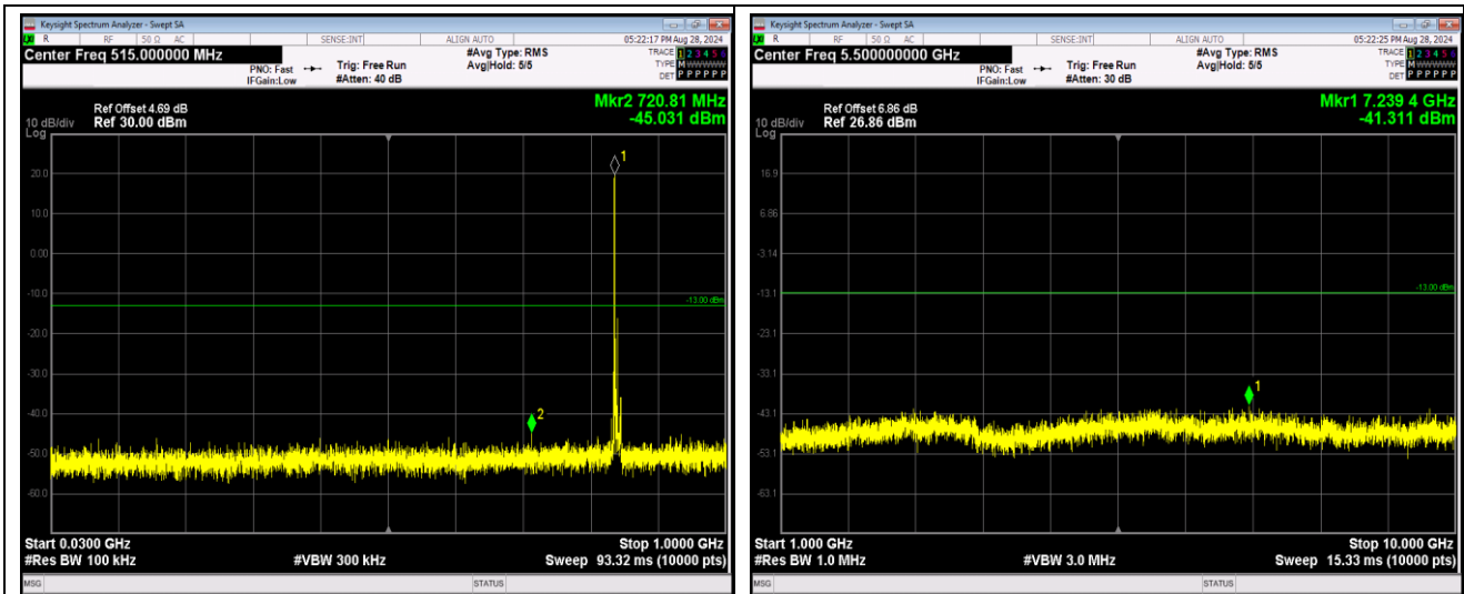
Band5-10MHz-64QAM-20450-1RB#0-Range1:30~1000MHz
