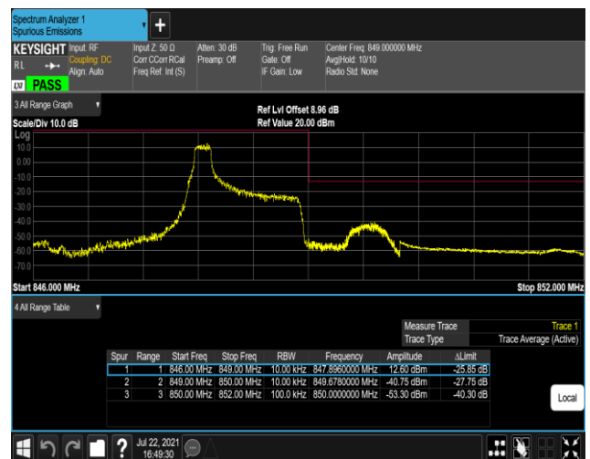
Band5-1.4MHz-QPSK-20643-6RB#0
