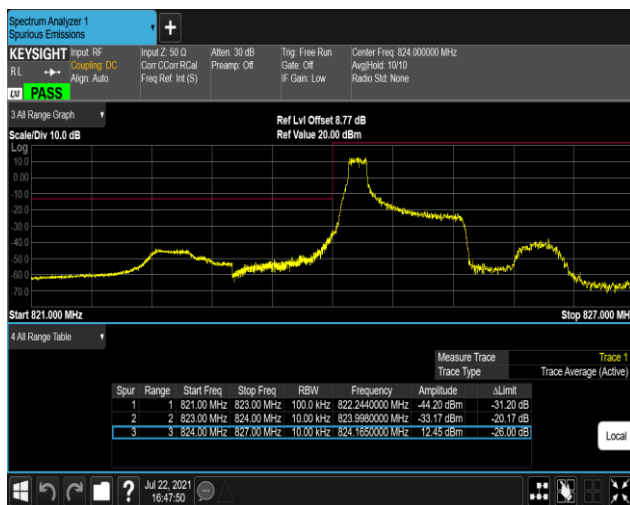
Band5-1.4MHz-QPSK-20407-6RB#0
