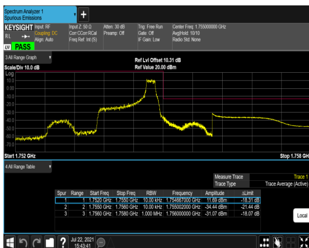
Band4-1.4MHz-16QAM-20393-1RB#5
