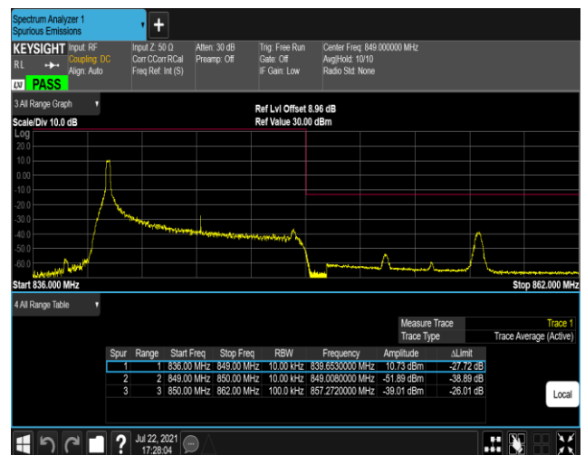
Band5-10MHz-QPSK-20600-50RB#0
