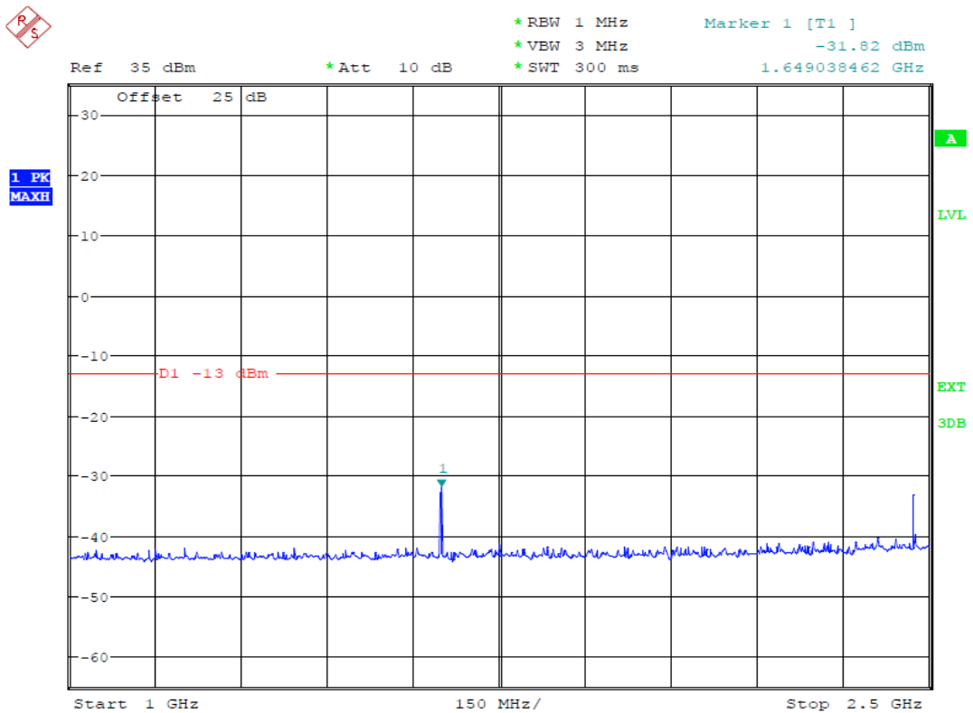
(Plot 4.7.1 A1: Channel 128: 824.20MHz @ Traffic @ GSM850)
