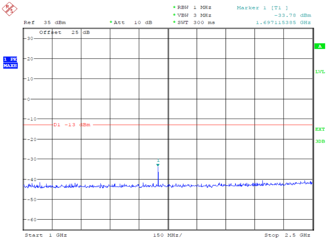
(Plot 4.7.3 A1: Channel 251: 848.80MHz @ Traffic @ GSM850)
