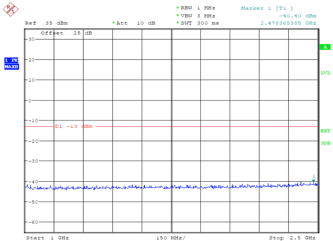
(Plot 4.7.4 A1: Idle @ GSM850)
